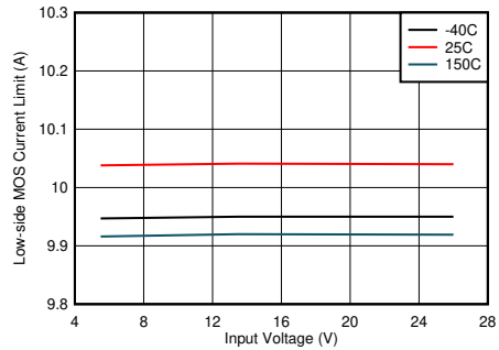
8-9. Low-side Current Limit vs Input Voltage
