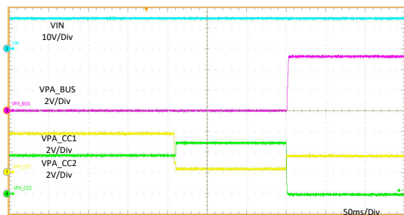
Figure 11-21. Rd Assert
