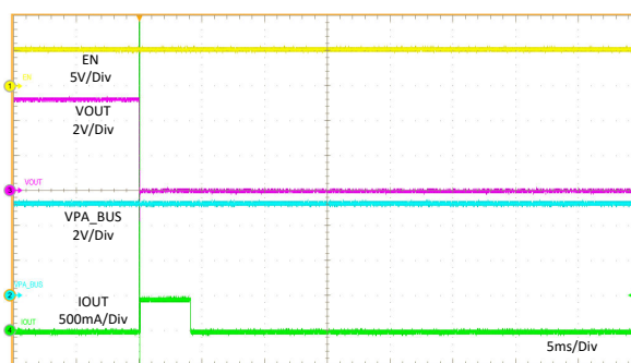
11-28. PA_CC2 Hot Short to GND
