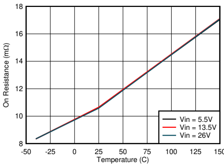
8-11. Low-side MOSFET on Resistance vs Junction Temperature
