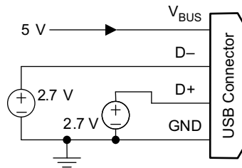
Figure 10-23. Divider 3 Mode
