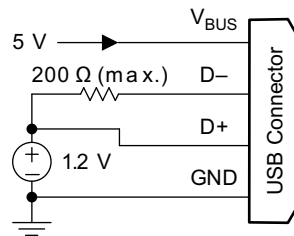
Figure 10-13. 1.2-V Mode
