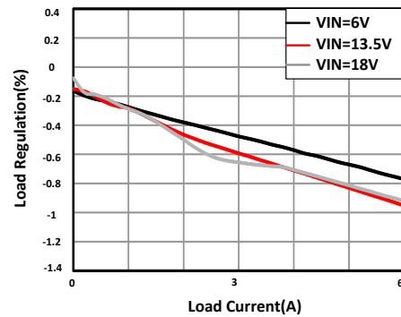
11-5. Load Regulation
