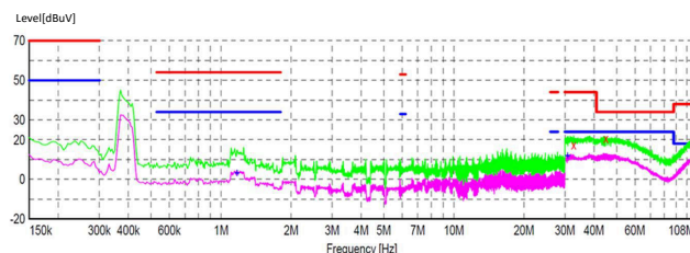
11-4. 400-kHz EMI Results (Without CM Filter)
