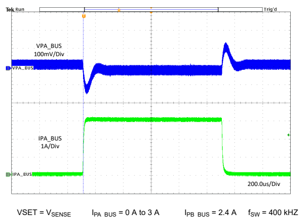
11-7. Load Transient Without Cable Compensation
