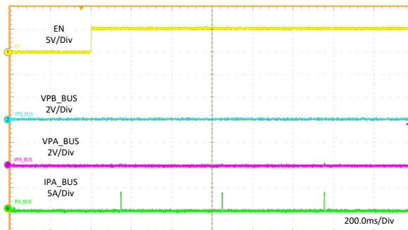
11-22. Enable Into Short
