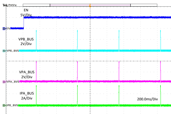
11-22. Enable Into Short
