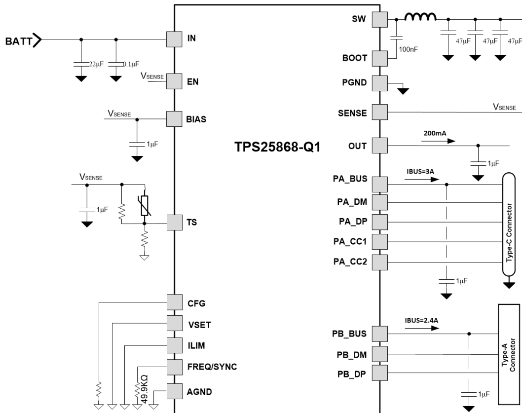
図 11-1. TPS25868-Q1 Typical Application Circuit for 400-kHz f_{sw}
