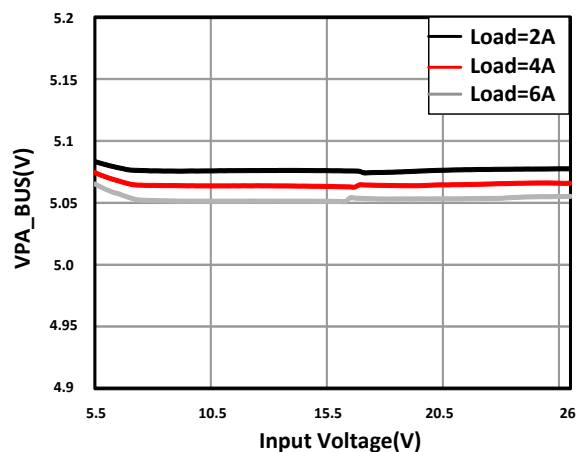
11-12. Dropout Characteristic
