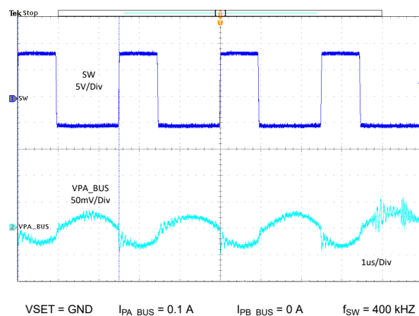
11-14. 100-mA Output Ripple
