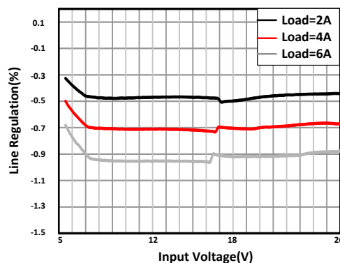
11-6. Line Regulation
