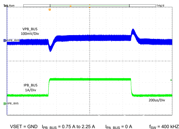
11-11. Load Transient With Cable Compensation
