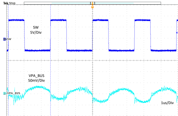
11-15. No Load Output Ripple
