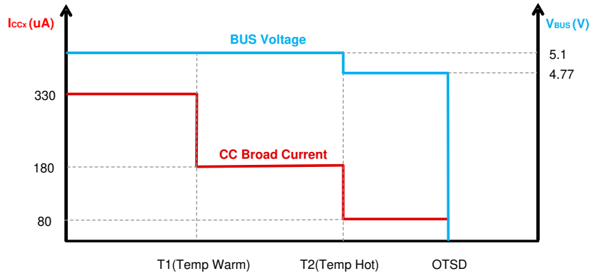
FIG 10-11. TPS2586x-Q1 Behavior When Trigger Temp Warm and Hot threshold
