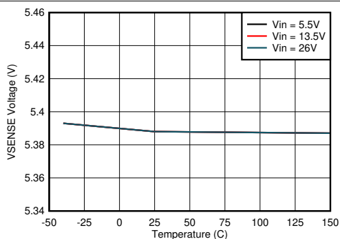
FIG 8-5. V_{\text{SENSE}} Voltage vs Junction Temperature
