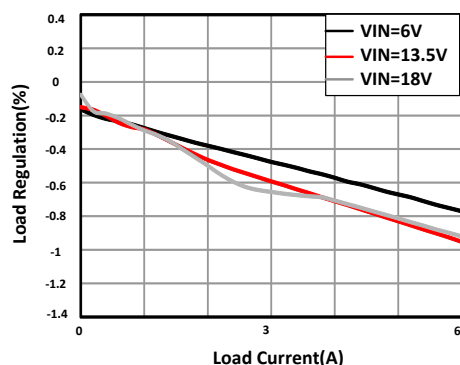
11-5. Load Regulation
