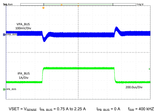
11-9. Load Transient Without Cable Compensation
