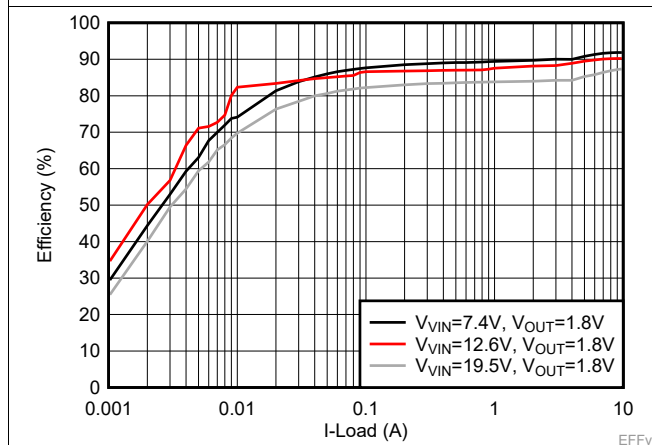
Figure 5. Efficiency Curve, V_{out}=1.8V
