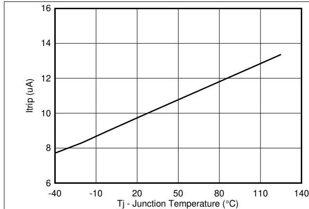
Figure 1. Trip Current Vs Temperature
