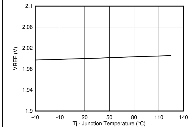
Figure 3. VREF Voltage Vs Temperature, I_{VREF}=0A
