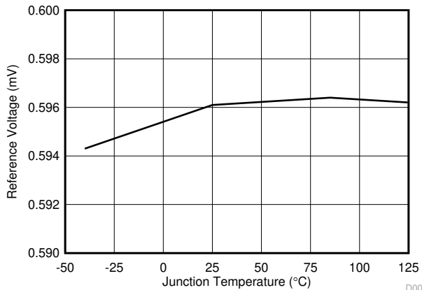
6-5. Reference Voltage vs Junction Temperature
