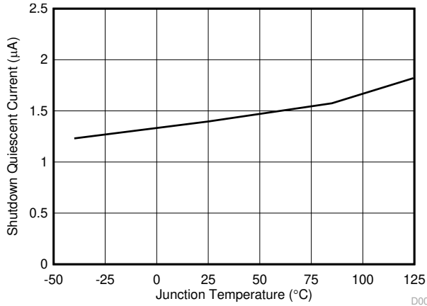
6-1. Shutdown Quiescent Current vs Junction Temperature
