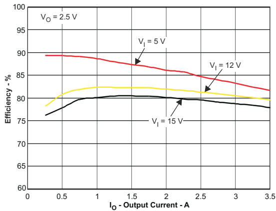
図 8-2. TPS54332 Efficiency
