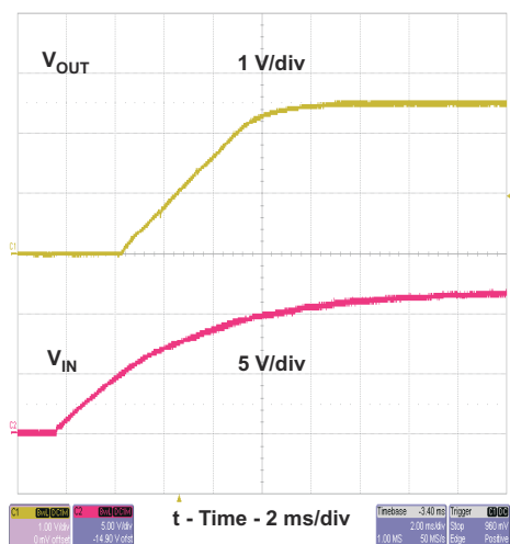
図 8-10. TPS54332 Start-Up
