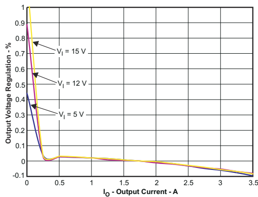
図 8-4. TPS54332 Load Regulation
