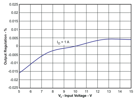
図 8-5. TPS54332 Line Regulation
