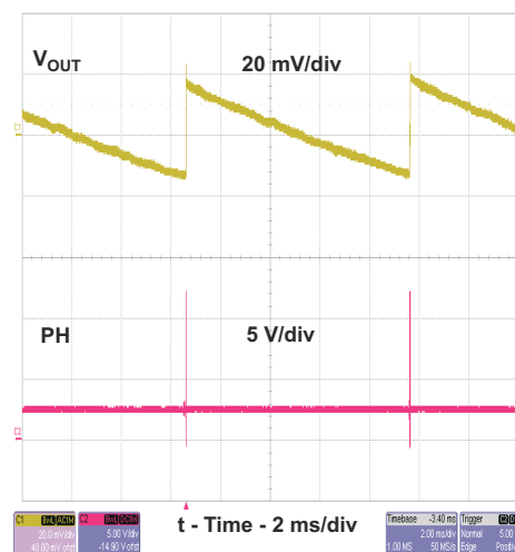
図 8-11. TPS54332 Output Ripple during Eco-mode Operation
