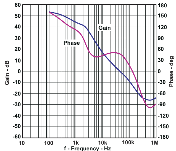
図 8-7. TPS54332 Loop Response
