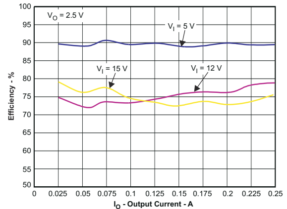
図 8-3. TPS54332 Low-Current Efficiency
