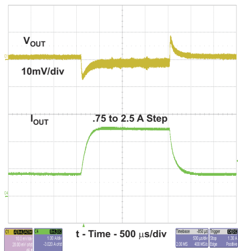
図 8-6. TPS54332 Transient Response
