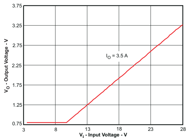
Figure 6-9. Typical Minimum Output Voltage vs Input Voltage
