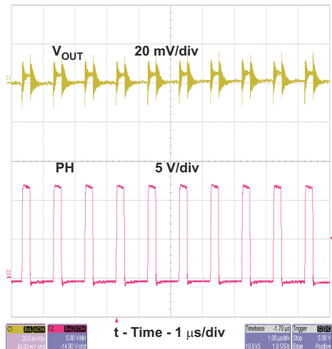
図 8-8. TPS54332 Output Ripple
