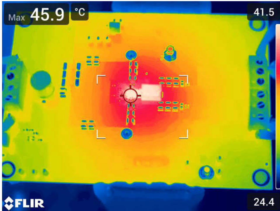
図 7-24. Thermal Image at 25°C Ambient
