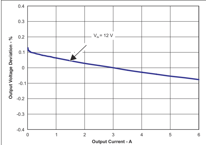
Figure 8-10. Load Regulation
