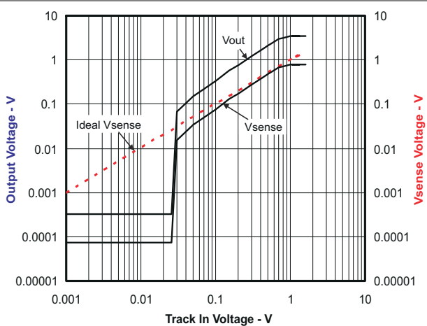
Figure 8-11. Tracking Performance
