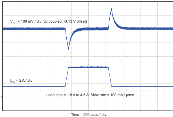
Figure 8-2. Load Transient
