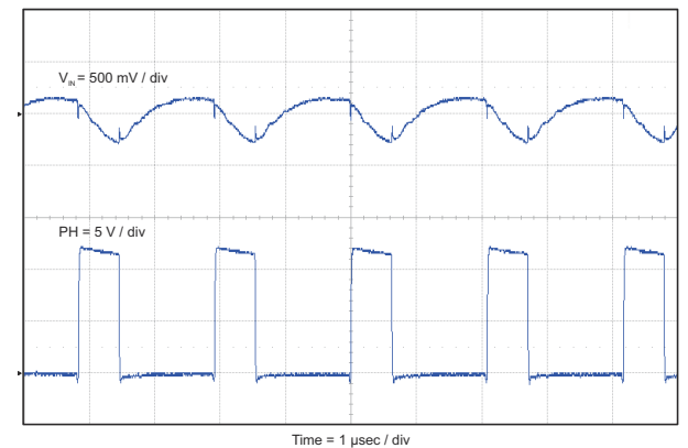
Figure 8-7. Input Voltage Ripple With Full Load
