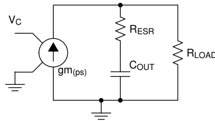
Figure 7-5. Simplified Small Signal Model for Peak Current Mode Control
