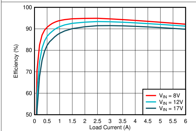
Figure 8-12. Efficiency vs Load Current
