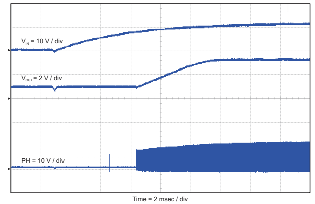
Figure 8-5. Start-Up With PRE-BIAS
