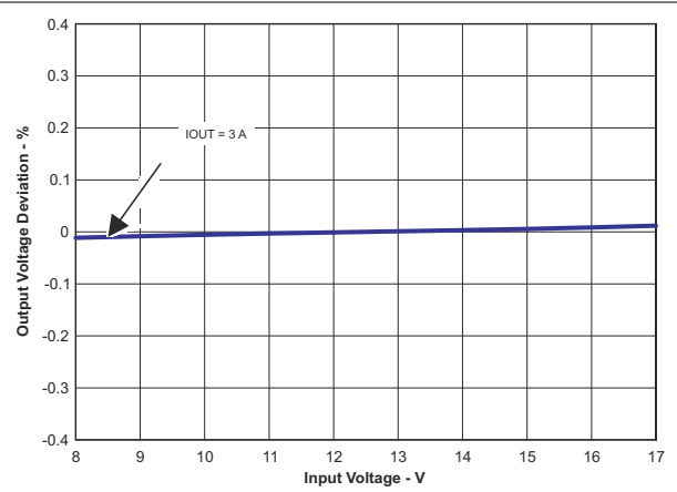
Figure 8-9. Line Regulation
