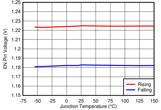
Figure 6-8. EN Pin UVLO Threshold vs Temperature
