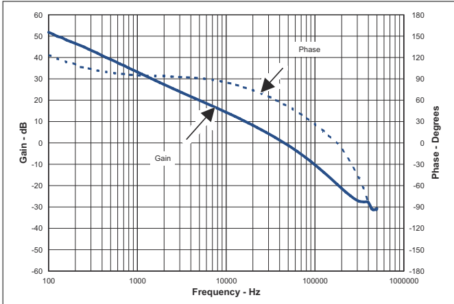
Figure 8-8. Closed Loop Response
