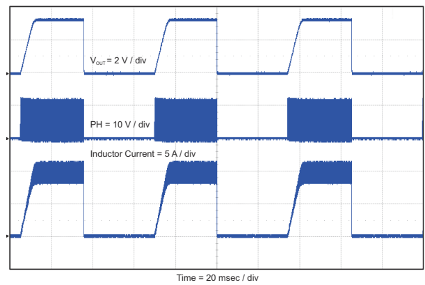
Figure 8-17. Hiccup Mode Current Limit
