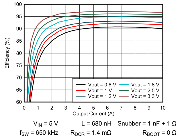
Figure 6-2. TPS546A24A Efficiency vs Output Current
