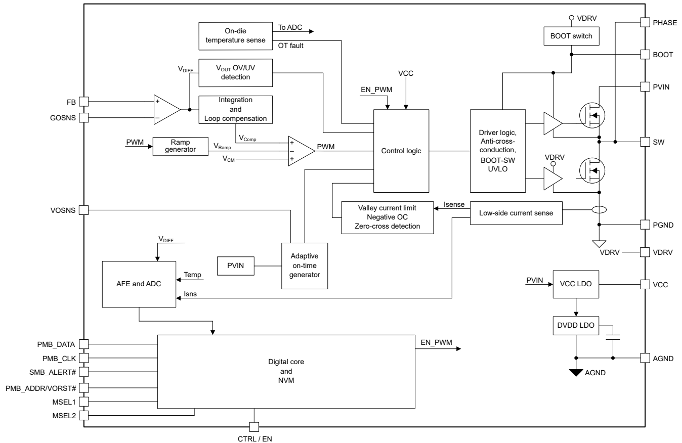
6-2. Block Diagram when External Feedback is Selected
