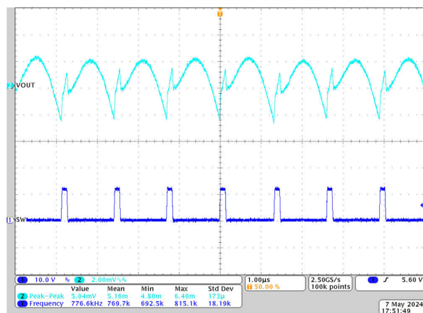
8-6. Output Voltage Ripple, 1.2V Vout, 800kHz FCCM, 25A Load
