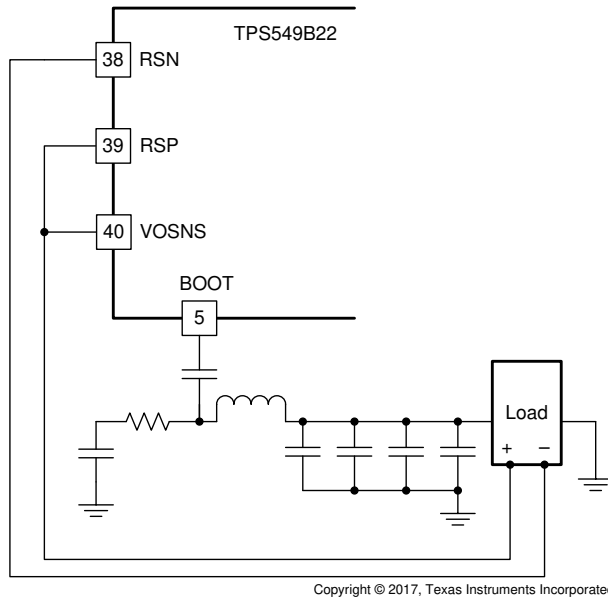
FIG 6-7. Remote Sensing Without Feedback Resistors
