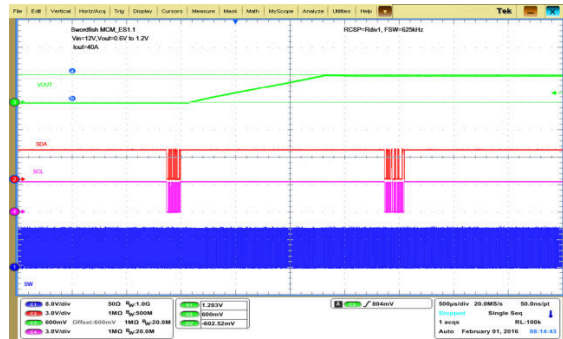
図 8-5. VOUT Command
