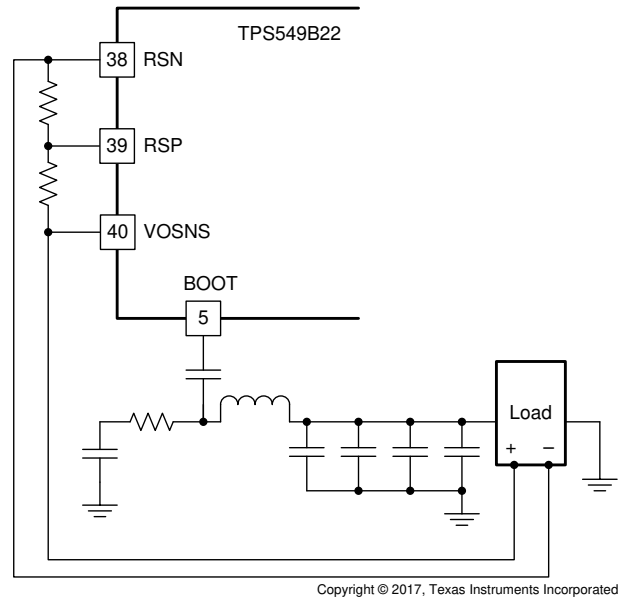
FIG 6-8. Remote Sensing With Feedback Resistors
