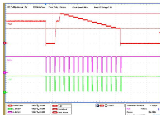
Figure 16. 6 Sequenced Events – I2C Write/Read with PEC
