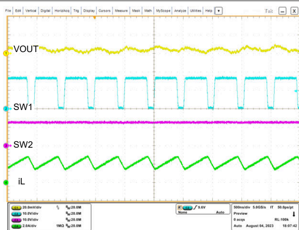
8-2. Switching Waveforms in V_{IN} = 16\text{ V} , V_{OUT} = 12\text{ V} , I_O = 2\text{ A} , FPWM
