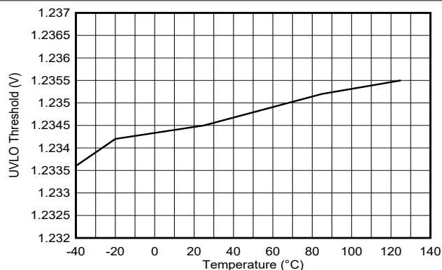
FIG 6-20. ENABLE/UVLO Rising Threshold vs Temperature
