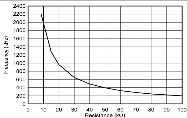
6-16. Switching Frequency vs Setting Resistance
