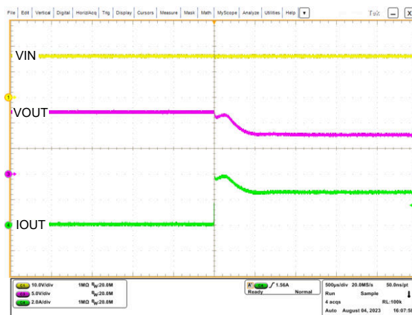
8-12. Output Current Limit Waveforms in V_{IN} = 16\text{ V} , V_{OUT} = 12\text{ V} , R_{LOAD} = 3\ \Omega , R_{SNS} = 20\text{ m}\Omega , FPWM
