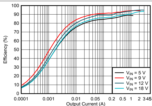
6-14. Efficiency vs Output Current, V_{OUT} = 12\text{ V} , f_{sw} = 2\text{ MHz} , PFM
