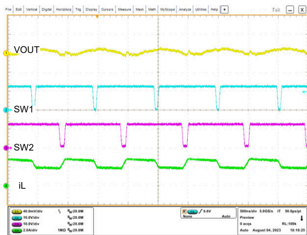
8-4. Switching Waveforms in V_{IN} = 12\text{ V} , V_{OUT} = 12\text{ V} , I_O = 2\text{ A} , FPWM
