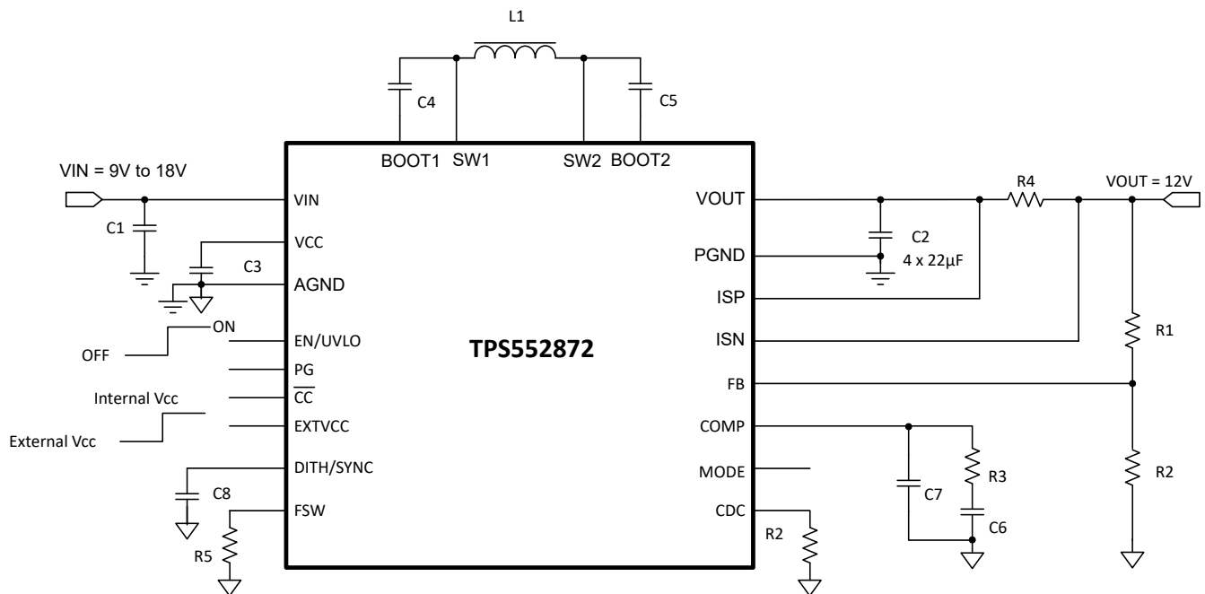
図 8-1. 12-V Power Supply With 9-V to 18-V Input Voltage
