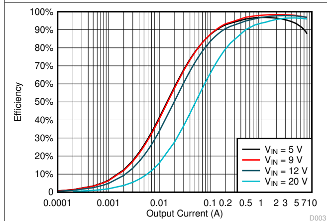
6-3. Efficiency vs Output Current, V_{OUT} = 9\text{ V} , FPWM
