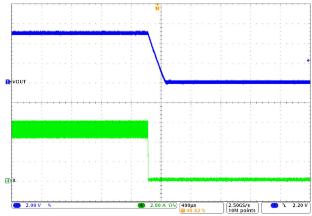
8-9. Shutdown Waveforms in V_{IN} = 12\text{ V} , V_{OUT} = 5\text{ V} , I_{OUT} = 5\text{ A} , FPWM
