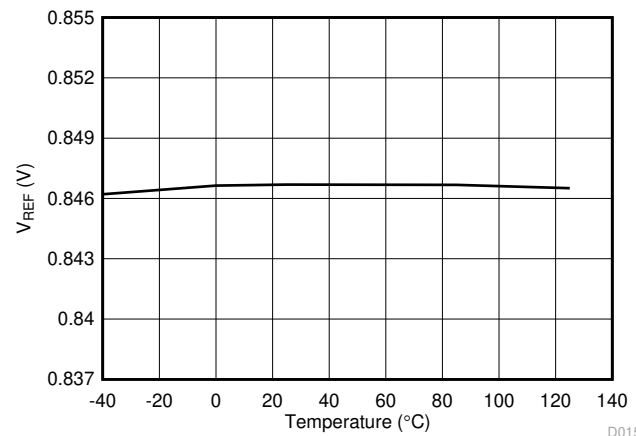
6-15. Reference Voltage vs Temperature ( V_{REF} = 0.846\text{ V} )
