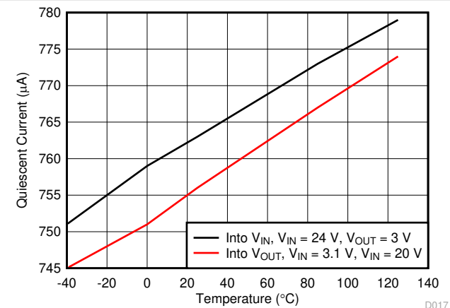
6-17. Quiescent Current vs Temperature
