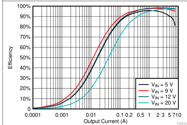
6-5. Efficiency vs Output Current, V_{OUT} = 12\text{ V} , FPWM
