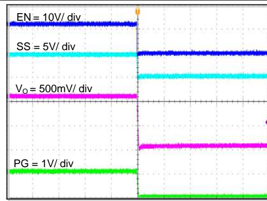
⊗ 46. TPS563210A Shut Down Relative To EN
