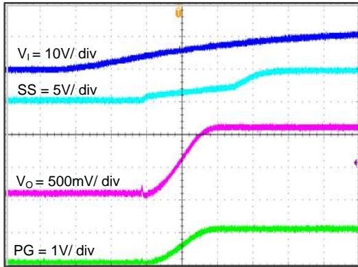
⊗ 43. TPS563210A Start Up Relative To V_1
