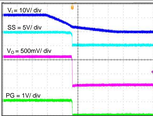
⊗ 45. TPS563210A Shut Down Relative To V_1
