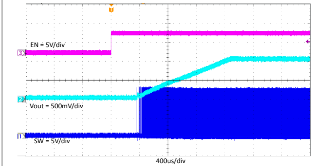
7-12. TPS563203 Enable on With 3A Loading
