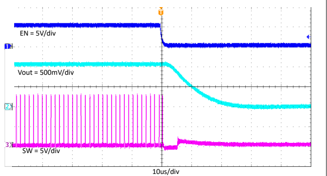
7-15. TPS563206 Enable off With 3A Loading
