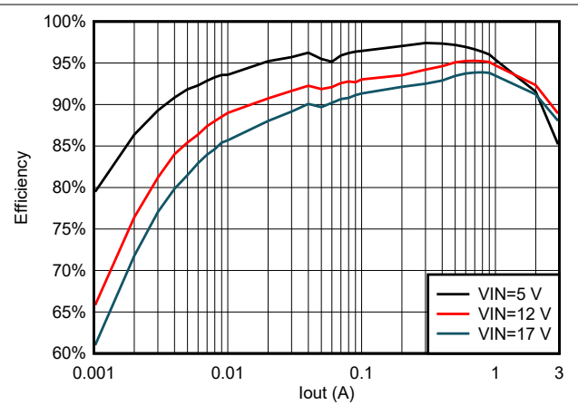
5-14. TPS563203 Efficiency at 3.3 Vout With 4.7 \mu H Inductor
