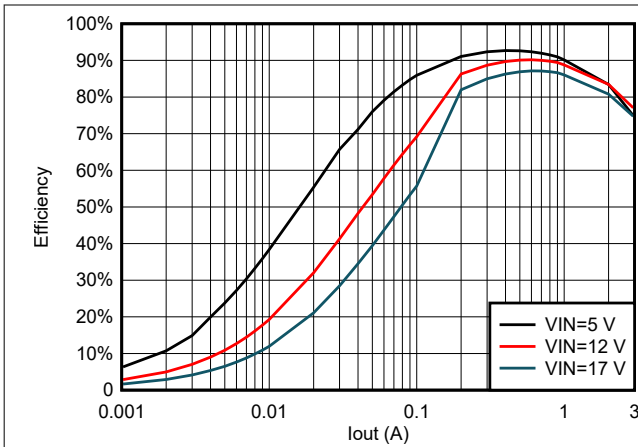
5-13. TPS563206 Efficiency at 1.05 Vout With 2.2 \mu H Inductor
