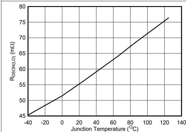
图 5-5. Low-Side R_{dson}
