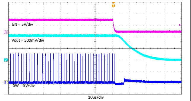
7-13. TPS563203 Enable off With 3A Loading
