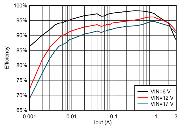
5-16. TPS563203 Efficiency at 5 Vout With 4.7 \mu H Inductor
