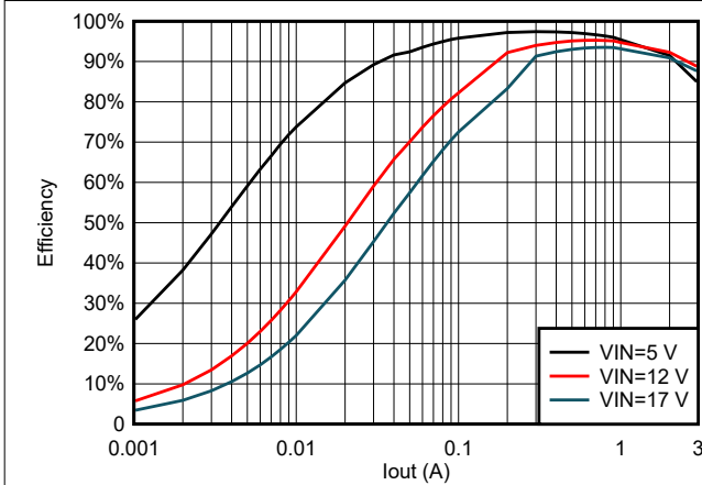
5-15. TPS563206 Efficiency at 3.3 Vout With 4.7 \mu H Inductor
