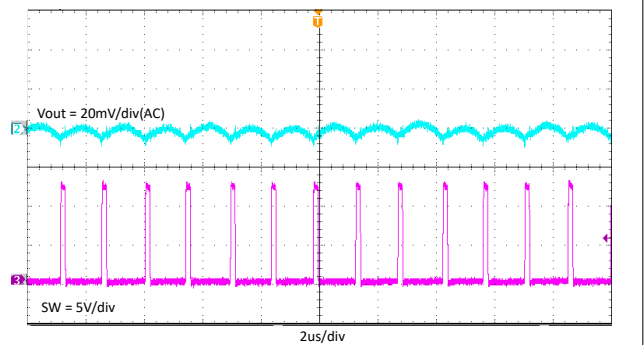
7-11. TPS563206 Output Voltage Ripple With 3A Loading
