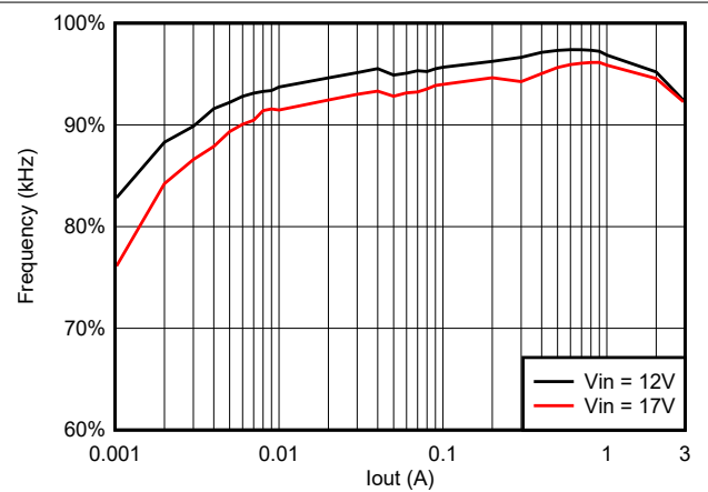
5-18. TPS563203 Efficiency at 7 Vout With 6.8 \mu H Inductor
