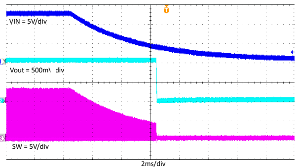
7-19. TPS563206 Power off With 3A Loading
