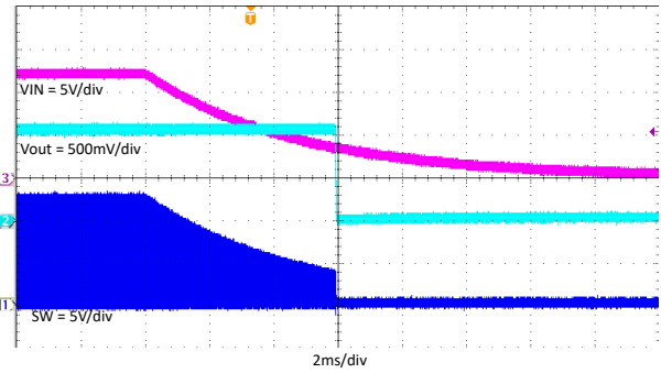
7-17. TPS563203 Power off With 3A Loading
