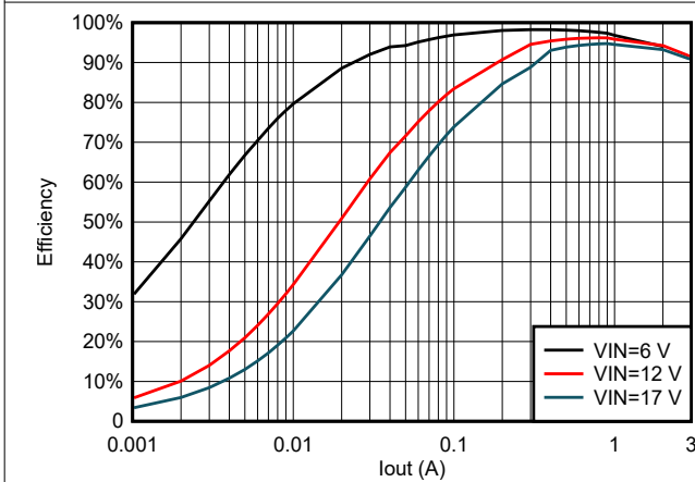
5-17. TPS563206 Efficiency at 5 Vout With 4.7 \mu H Inductor
