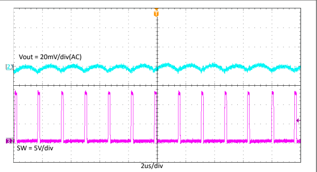
7-9. TPS563206 Output Voltage Ripple With 0.1A Loading
