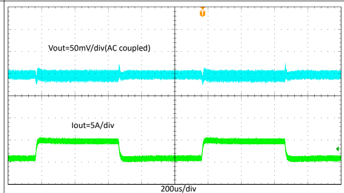
8-13. TPS565247 Transient Response with 0.5 A to 4.5 A by 2.5-A/ \mu s Load Step
