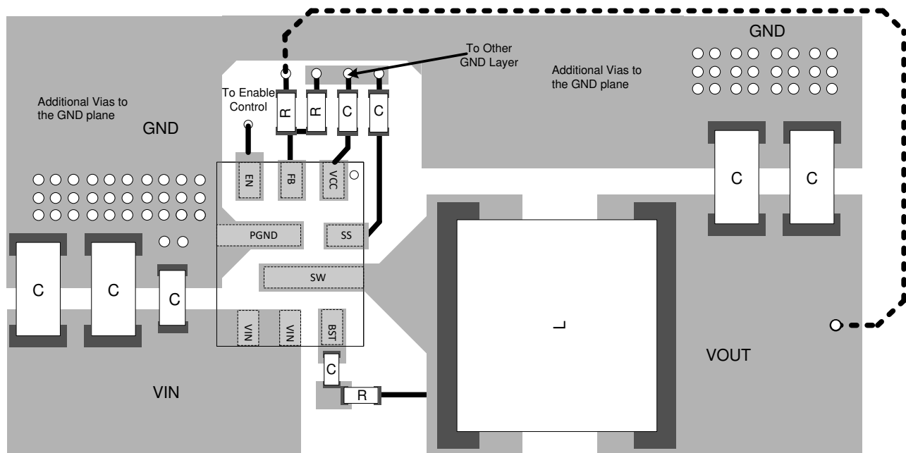
☒ 7-26. Top-Layer Layout
