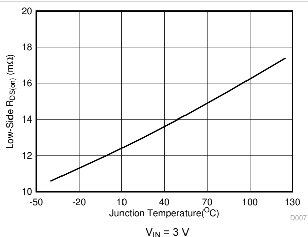
Figure 5-10. Low-Side R_{DS(on)} vs Junction Temperature
