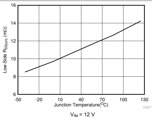
Figure 5-8. Low-Side R_{DS(on)} vs Junction Temperature
