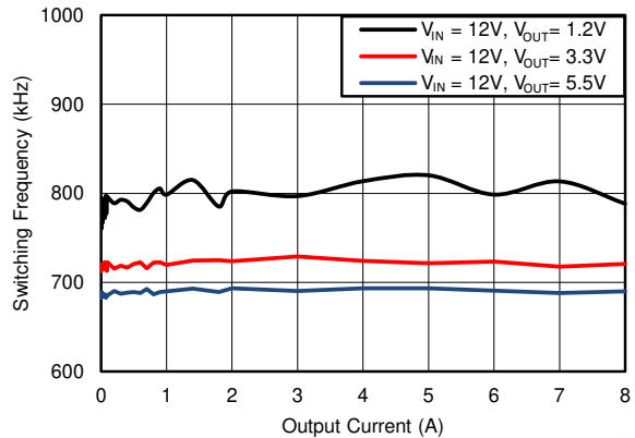
6-18. F_{SW} Load Regulation, Mode = FFCM, F_{SW} = 800\text{kHz}
