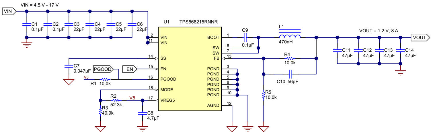
図 8-1. Application Schematic
