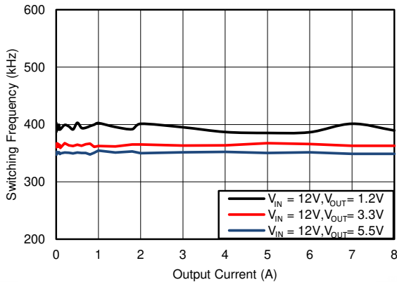
6-17. F_{SW} Load Regulation, Mode = FFCM, F_{SW} = 400\text{kHz}
