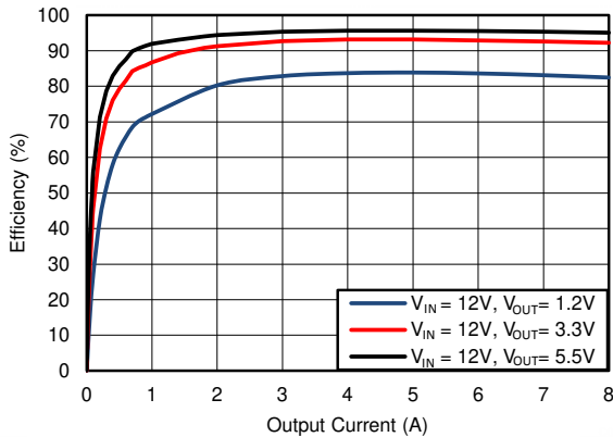
6-15. Efficiency, Mode = FFCM, F_{SW} = 1200\text{kHz}
