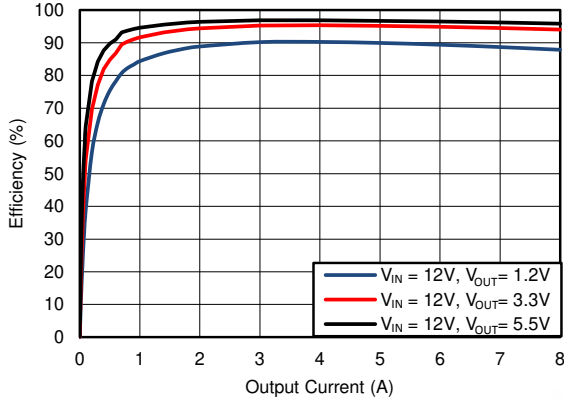
6-13. Efficiency, Mode = FFCM, F_{SW} = 400\text{kHz}
