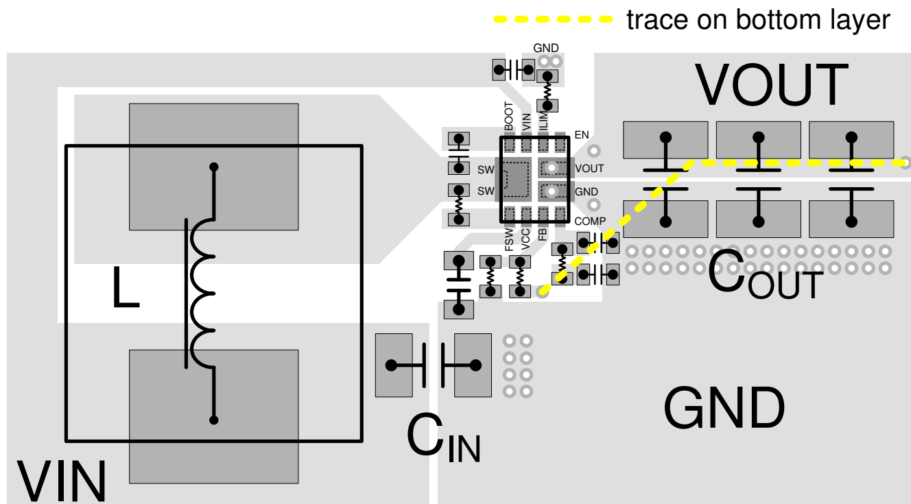
✎ 11-1. Layout Example
