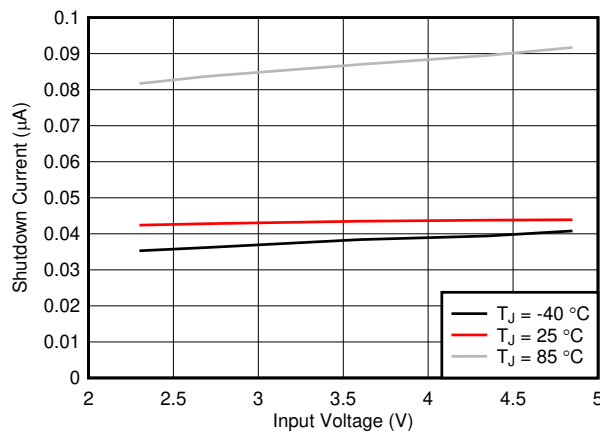
FIG 7-9. Shutdown Current vs Input Voltage
