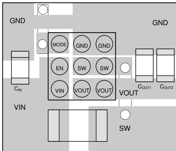
✎ 10-1. Recommended Layout
