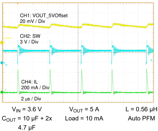
9-2. Steady 10 mA
