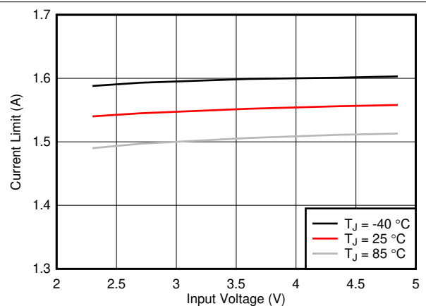
FIG 7-12. DC Startup Current Limit vs Input Voltage
