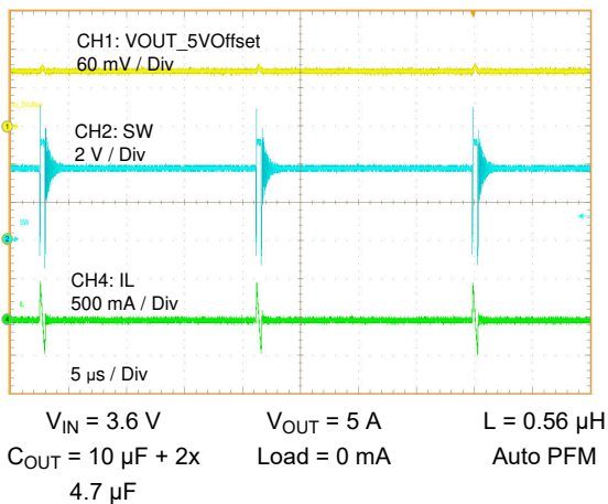
9-4. Steady Ultrasonic Mode
