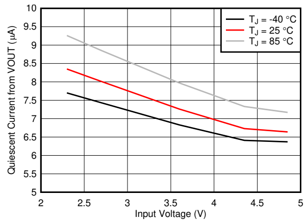
FIG 7-8. Quiescent Current (from VOUT) vs Input Voltage
