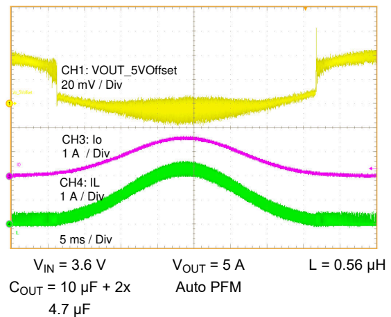
9-5. Load Sweep
