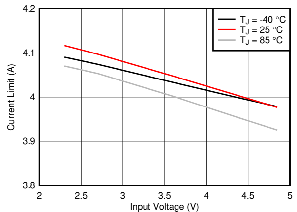
FIG 7-10. Current Limit (Auto PFM) vs Input Voltage
