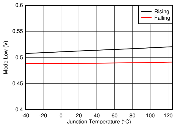
7-14. Mode Low Rising / Falling vs Temperature
