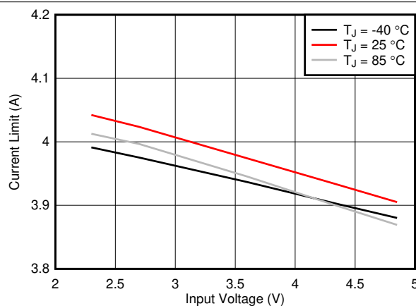
FIG 7-11. Current Limit (Forced PWM) vs Input Voltage
