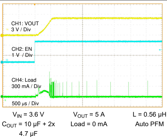
9-6. Start-up by EN
