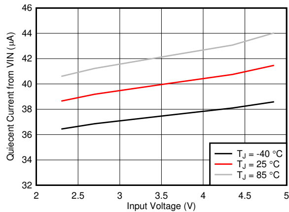
FIG 7-7. Quiescent Current (from VIN) vs Input Voltage
