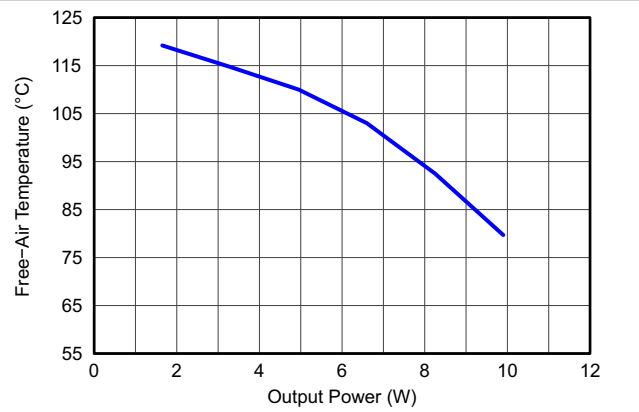
9-37. Typical Operation In Power Save Mode
