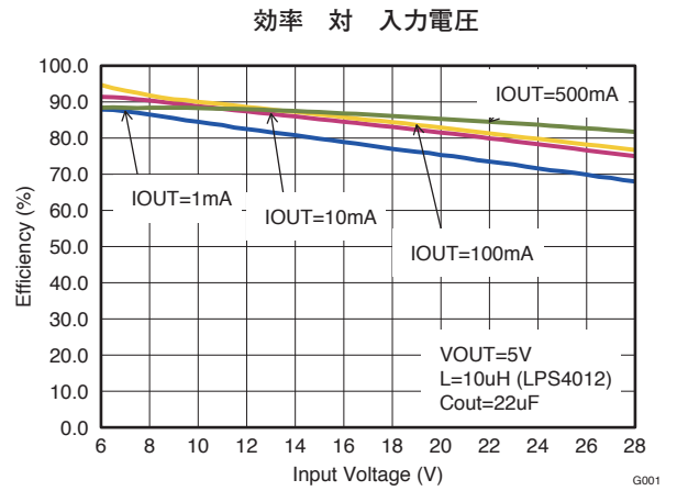
図 6. Vout = 5V
