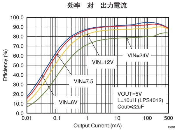
図 5. Vout = 5V
