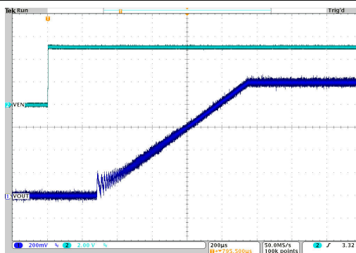
10-53. Start-Up Timing
