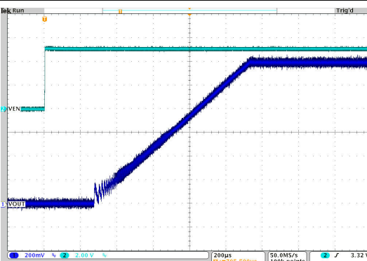
10-52. Start-Up Timing
