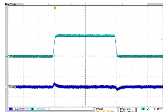
10-35. Line Transient Response
