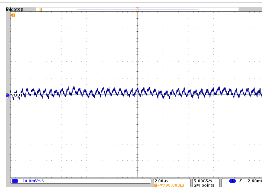
10-45. Output Voltage Ripple
