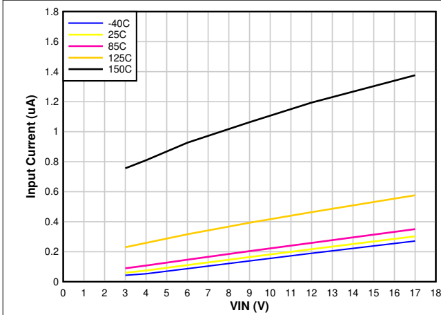
Figure 6-3. Typical Shutdown Current
