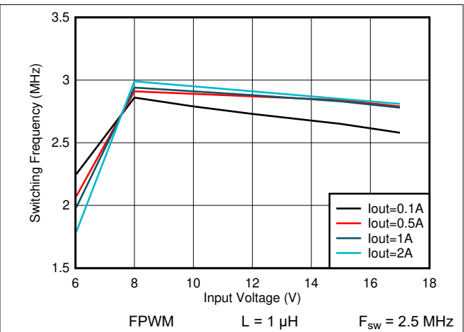
Figure 8-26. Switching Frequency vs Input Voltage V OUT = 5 V
