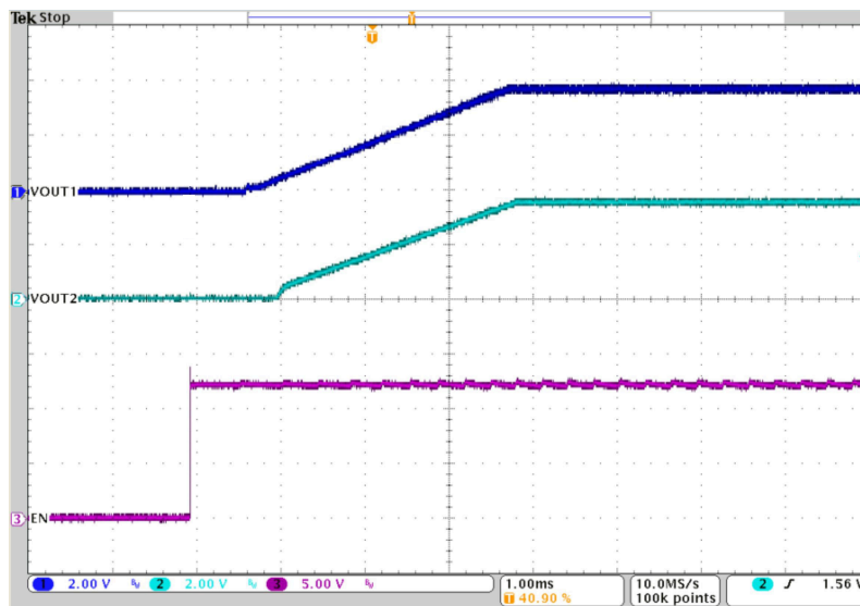
Figure 8-85. Tracking
