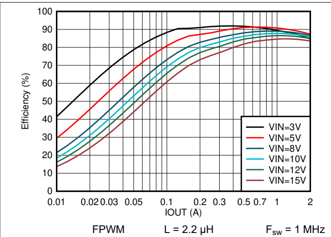
Figure 8-20. Efficiency vs Output Current V_{OUT} = 1.2\text{ V}
