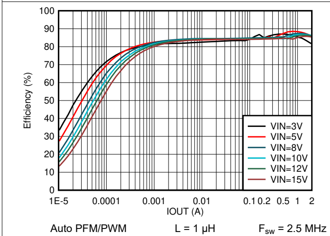
Figure 8-21. Efficiency vs Output Current V_{OUT} = 1.2\text{ V}
