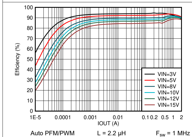
Figure 8-15. Efficiency vs Output Current V OUT = 1.8 V
