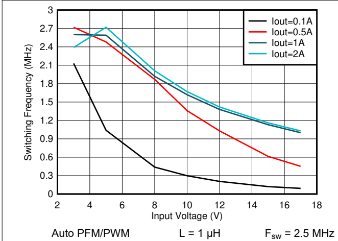
Figure 8-33. Switching Frequency vs Input Voltage V_{\text{OUT}} = 1.8 \text{ V}
