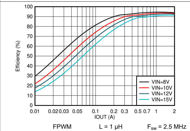
Figure 8-10. Efficiency vs Output Current V OUT = 5 V
