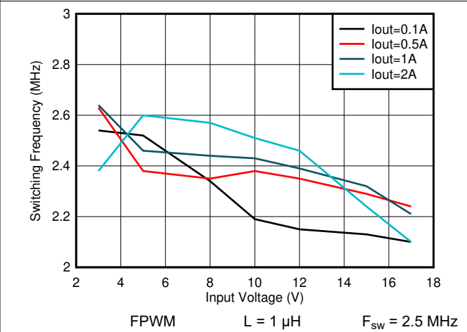
Figure 8-34. Switching Frequency vs Input Voltage V_{\text{OUT}} = 1.8 \text{ V}
