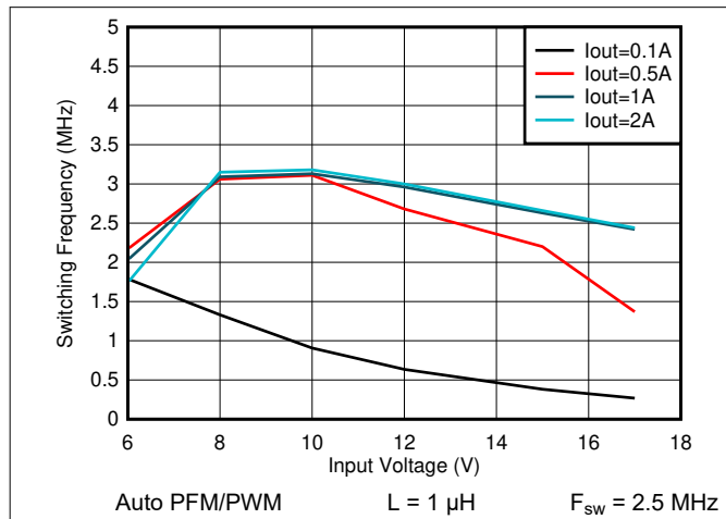
Figure 8-25. Switching Frequency vs Input Voltage V OUT = 5 V
