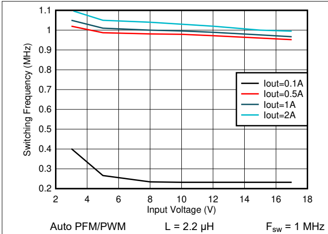
Figure 8-31. Switching Frequency vs Input Voltage V_{\text{OUT}} = 1.8 \text{ V}
