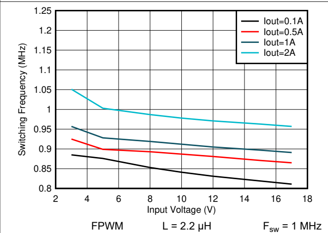
Figure 8-36. Switching Frequency vs Input Voltage V_{\text{OUT}} = 1.2 \text{ V}
