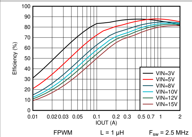
Figure 8-22. Efficiency vs Output Current V_{OUT} = 1.2\text{ V}
