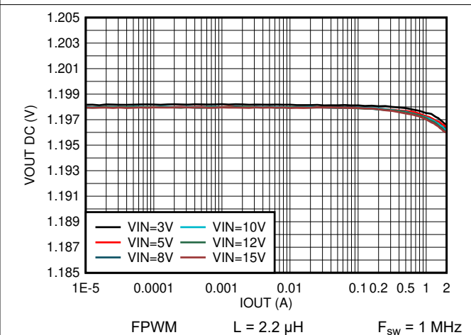
Figure 8-79. Output Voltage vs Output Current V_{OUT} = 1.2 V
