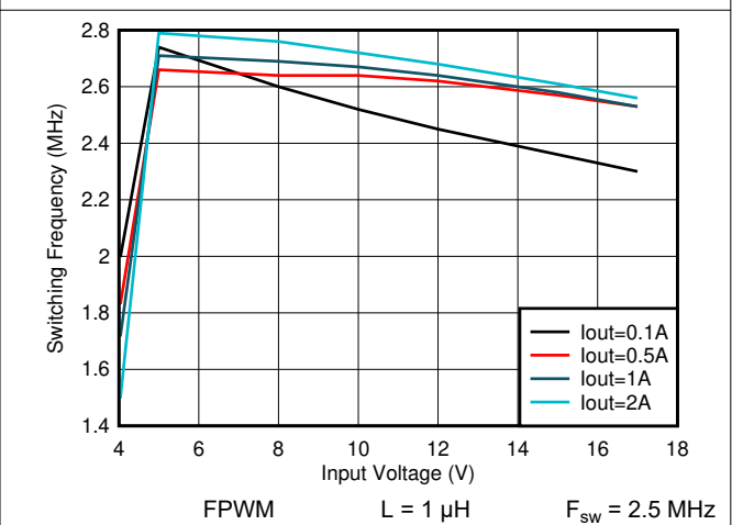
Figure 8-30. Switching Frequency vs Input Voltage V OUT = 3.3 V
