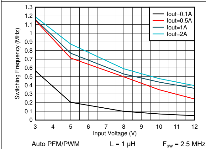
Figure 8-76. Switching Frequency vs Input Voltage V_{OUT} = 0.4 V
