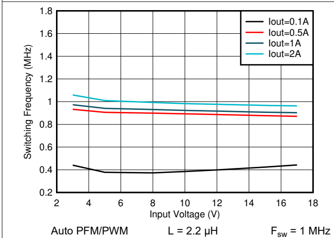
Figure 8-35. Switching Frequency vs Input Voltage V_{\text{OUT}} = 1.2 \text{ V}
