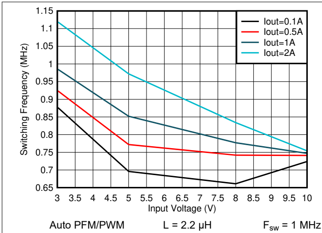
Figure 8-74. Switching Frequency vs Input Voltage V_{OUT} = 0.4 V
