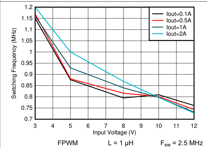
Figure 8-77. Switching Frequency vs Input Voltage V_{OUT} = 0.4 V
