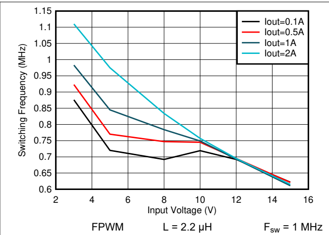
Figure 8-75. Switching Frequency vs Input Voltage V_{OUT} = 0.4 V
