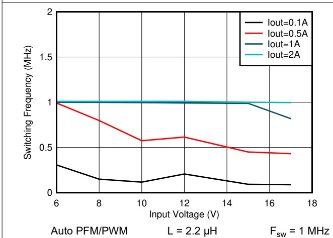
Figure 8-23. Switching Frequency vs Input Voltage V_{OUT} = 5\text{ V}
