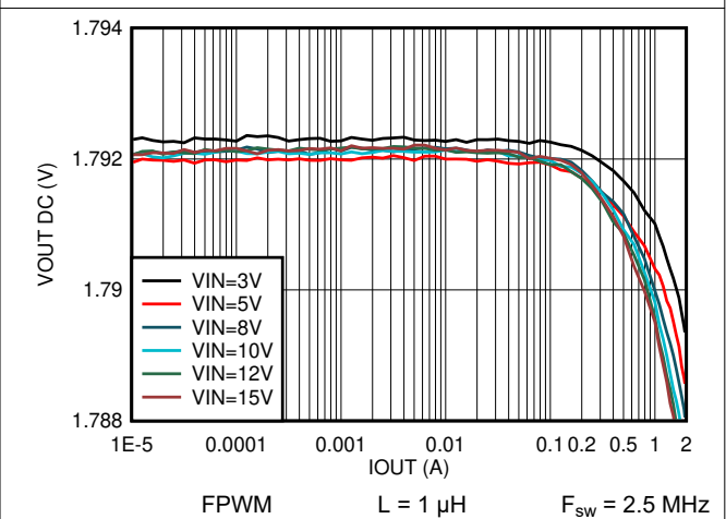
Figure 8-40. Output Voltage vs Output Current V OUT = 1.8 V
