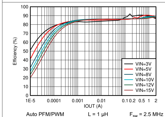
Figure 8-17. Efficiency vs Output Current V OUT = 1.8 V
