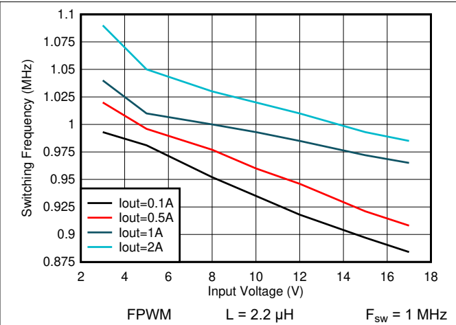
Figure 8-32. Switching Frequency vs Input Voltage V_{\text{OUT}} = 1.8 \text{ V}
