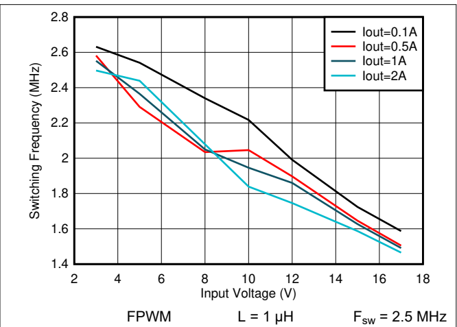
Figure 8-38. Switching Frequency vs Input Voltage V OUT = 1.2 V
