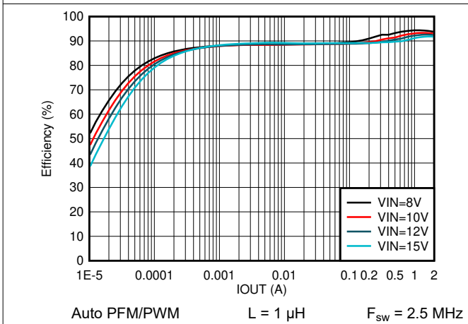
Figure 8-9. Efficiency vs Output Current V OUT = 5 V
