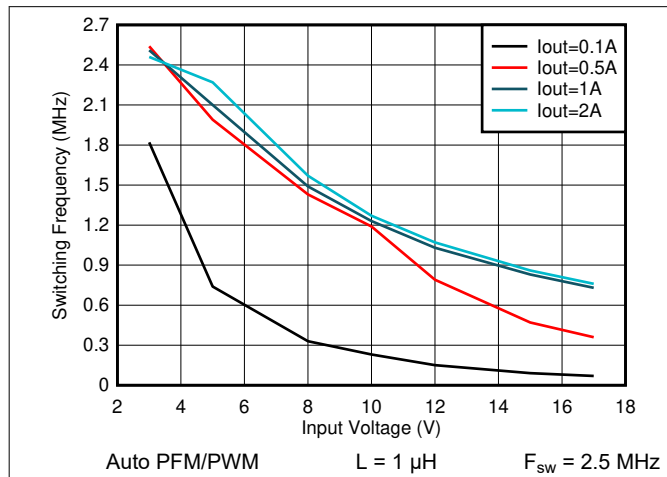
Figure 8-37. Switching Frequency vs Input Voltage V OUT = 1.2 V
