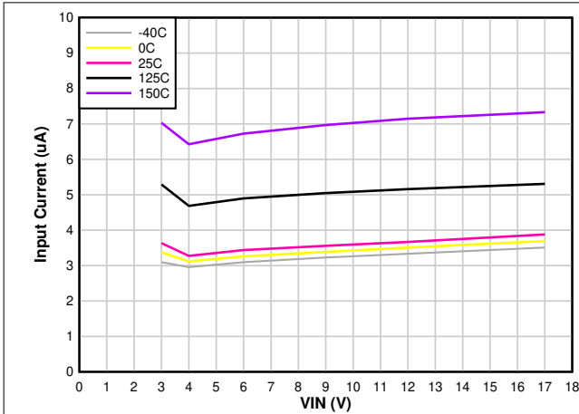
Figure 6-1. Typical Quiescent Current vs V_{IN}
