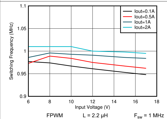
Figure 8-24. Switching Frequency vs Input Voltage V_{OUT} = 5\text{ V}
