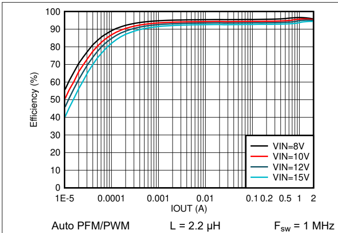
Figure 8-7. Efficiency vs Output Current V OUT = 5 V
