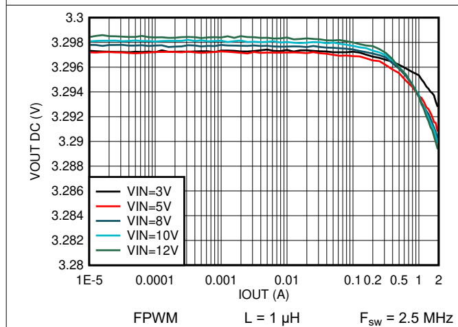
Figure 8-39. Output Voltage vs Output Current V OUT = 3.3 V
