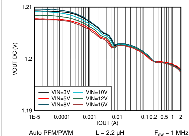
Figure 8-78. Output Voltage vs Output Current V_{OUT} = 1.2 V
