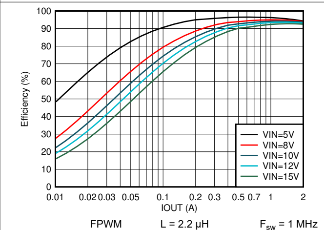
Figure 8-12. Efficiency vs Output Current V OUT = 3.3 V
