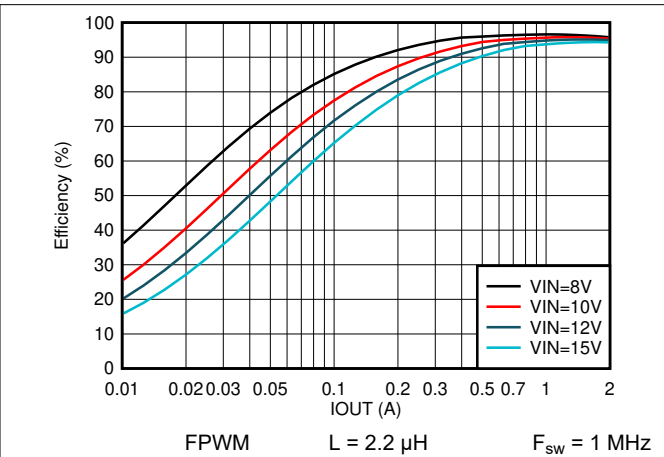
Figure 8-8. Efficiency vs Output Current V OUT = 5 V
