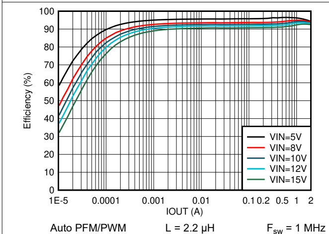
Figure 8-11. Efficiency vs Output Current V OUT = 3.3 V
