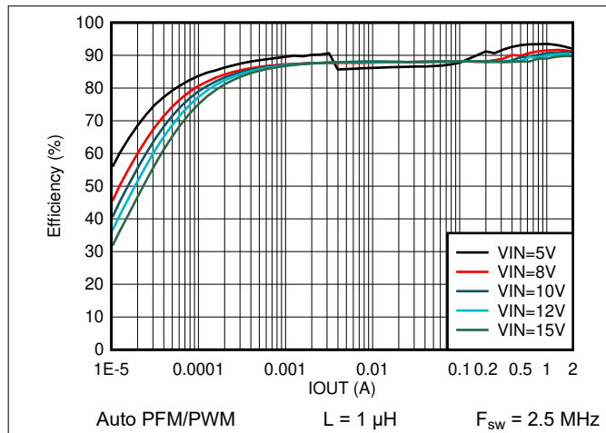
Figure 8-13. Efficiency vs Output Current V OUT = 3.3 V
