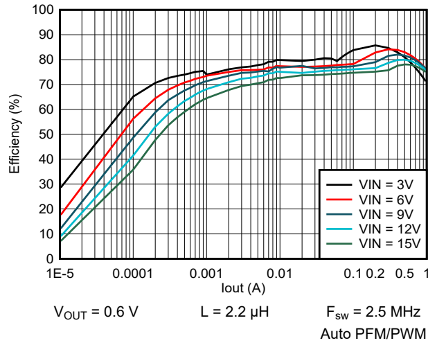
9-50. Efficiency vs Output Current
