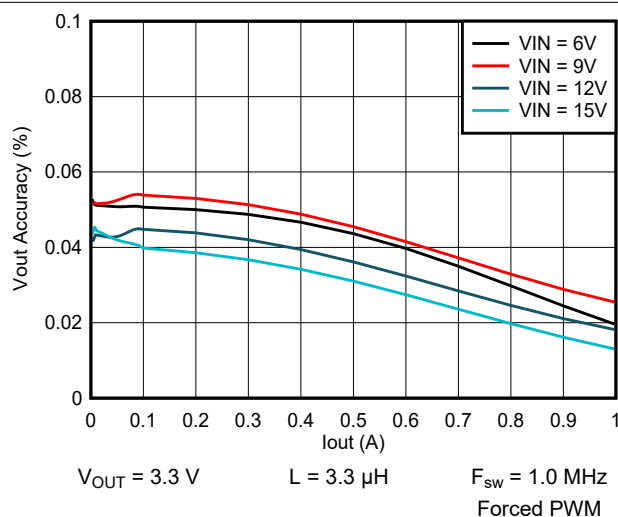
9-25. Output Voltage vs Output Current
