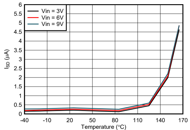
Figure 7-2. Shutdown Current vs Temperature
