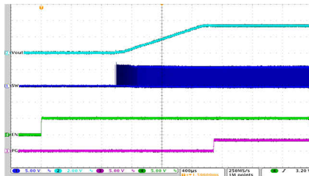
图 9-64. Start-Up Timing
