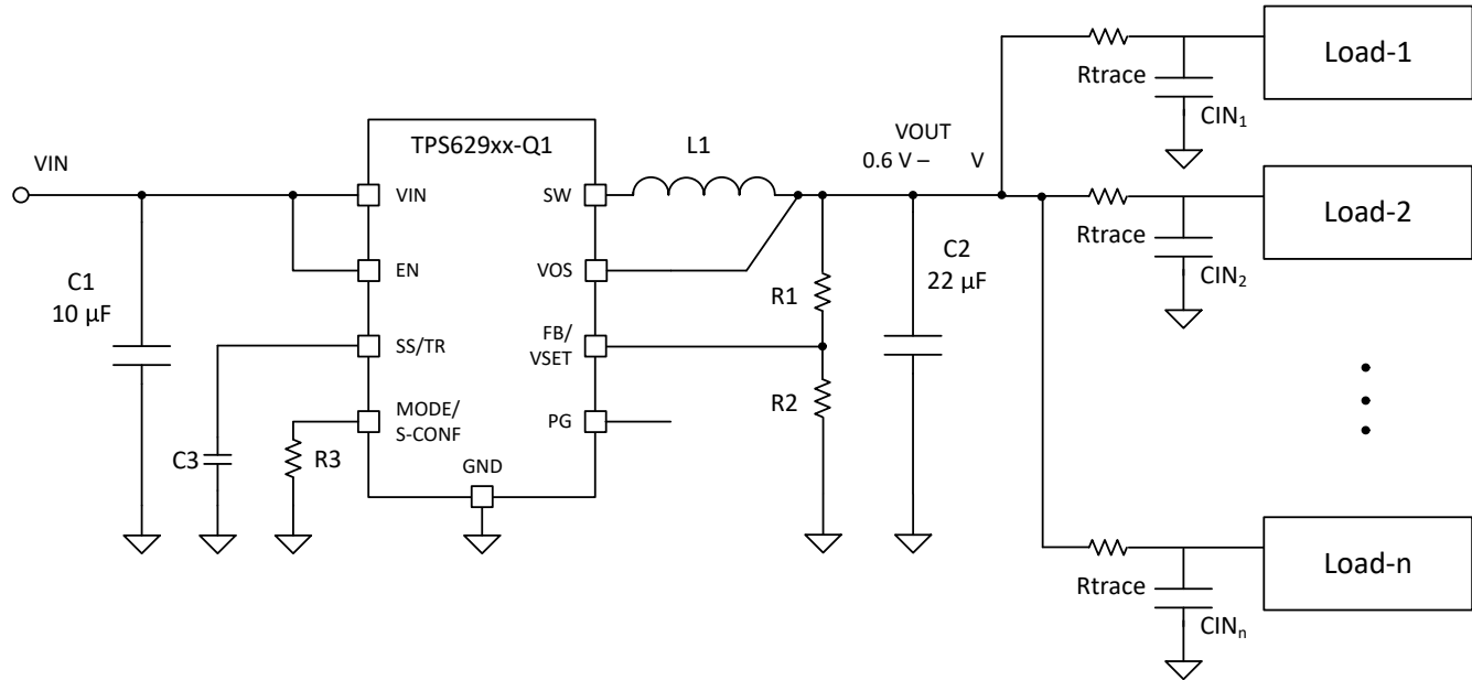
9-83. Multiple Loads
