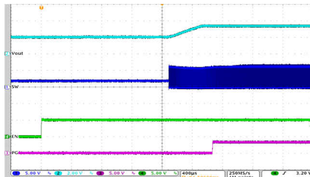
图 9-66. Start-Up Timing
