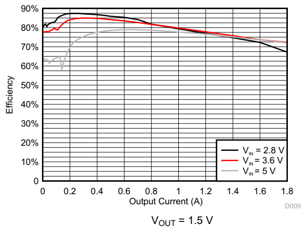
8-6. DCDC3 Efficiency
