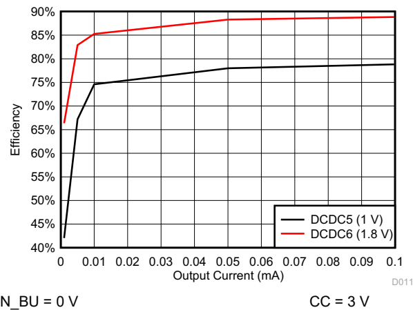
8-8. DCDC5/DCDC6 Efficiency
