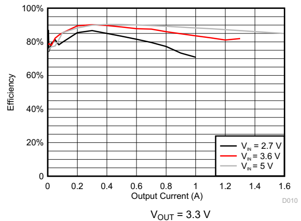
8-7. DCDC4 Efficiency
