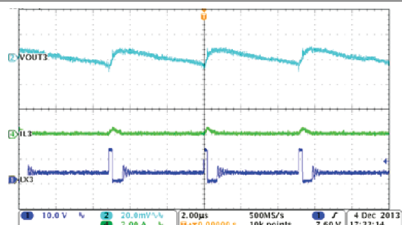
8-13. PSM Mode Buck3, Steady State Operation with Light Load
