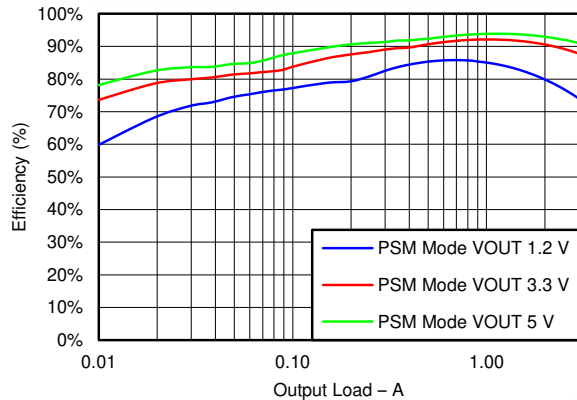
FIG 6-1. Buck1 Efficiency
