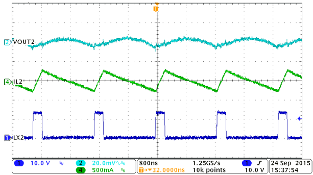
8-34. PWM Mode, Buck2, Steady State Operation with No Load
