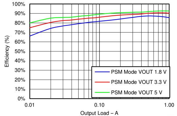
FIG 6-2. Buck2 Efficiency
