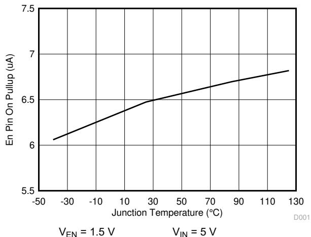
FIG 6-14. EN Pin Pullup Current vs Temperature
