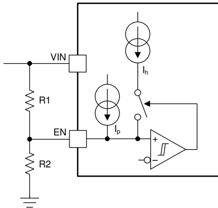
FIG 7-2. Adjustable V_{IN} UVLO
