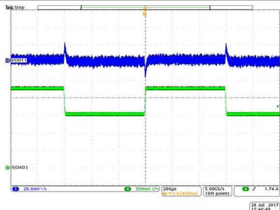
8-10. BUCK1 Load Transient
