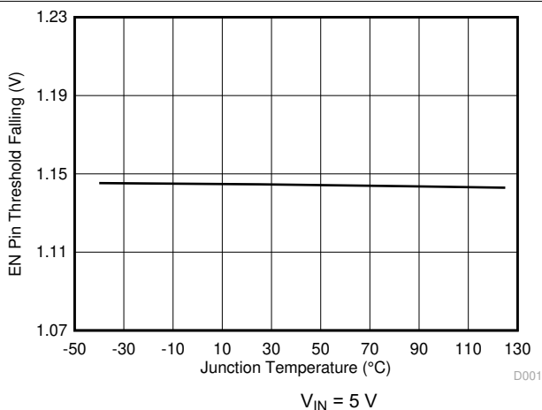
FIG 6-16. EN Pin Threshold Falling vs Temperature
