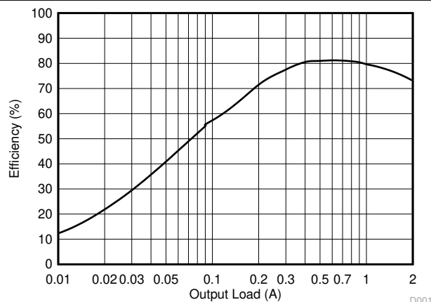
FIG 6-2. BUCK2 Efficiency
