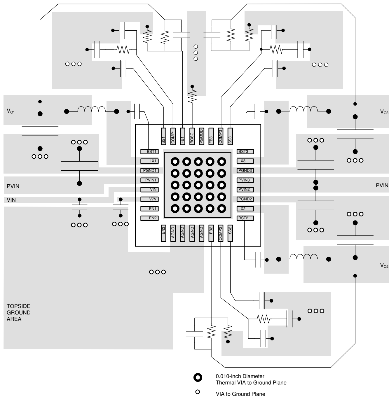
8-22. PCB Layout
