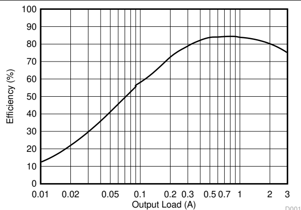
FIG 6-1. BUCK1 Efficiency
