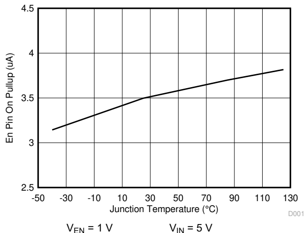
FIG 6-13. EN Pin Pullup Current vs Temperature
