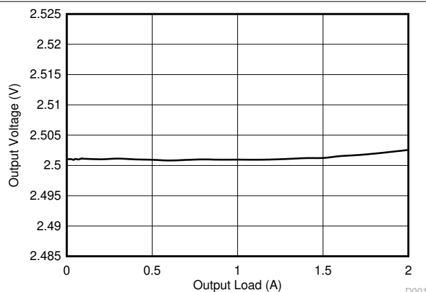
FIG 6-6. BUCK3, Load Regulation
