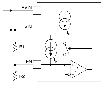
FIG 7-4. Adjustable V_{IN} and PV_{IN} UVLO
