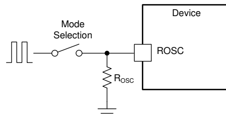
図 7-11. Works With Resistor Mode and Synchronization Mode
