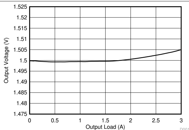
FIG 6-4. BUCK1, Load Regulation
