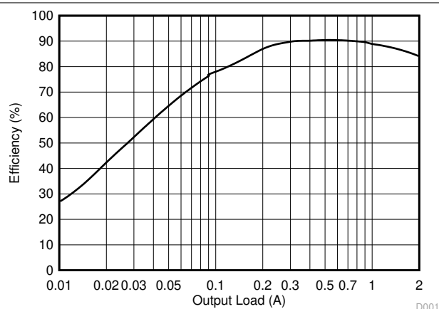
FIG 6-3. BUCK3 Efficiency
