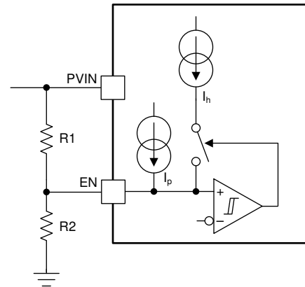
FIG 7-3. Adjustable PV_{IN} UVLO, V_{IN} > 4 V
