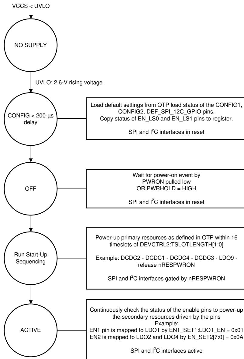
FIG 8-4. STARTUP Flow for CONFIG2 Pin Shorted to LDOAO
