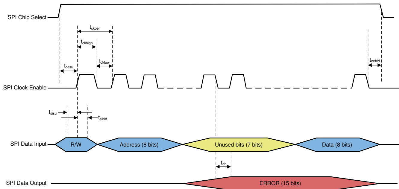
7-3. SPI Timing
