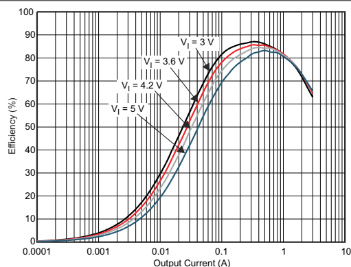
V_{OUT} = 0.9\text{ V} PWM Mode DFE252012P-1R0 T_A = 25^\circ\text{C}
