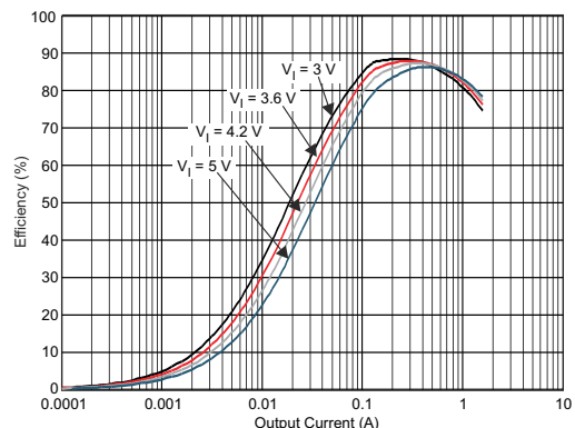
V_{OUT} = 1.1375\text{ V} DFE252012-1R0 PWM Mode T_A = 25^\circ\text{C}
