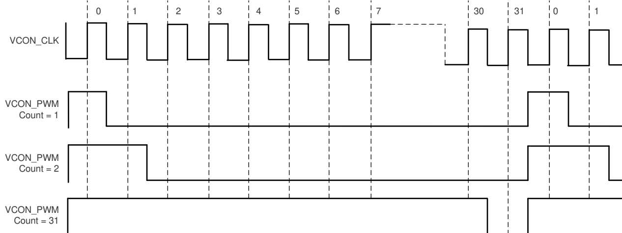
图 8-12. VCON Voltage Scaling Architecture
