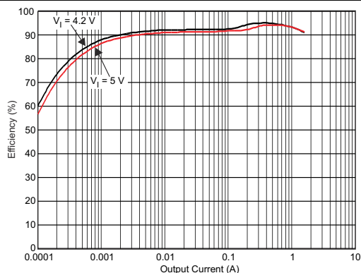
V_{OUT} = 3.2\text{ V} DFE25012-1R0 PFM Mode T_A = 25^\circ\text{C}
