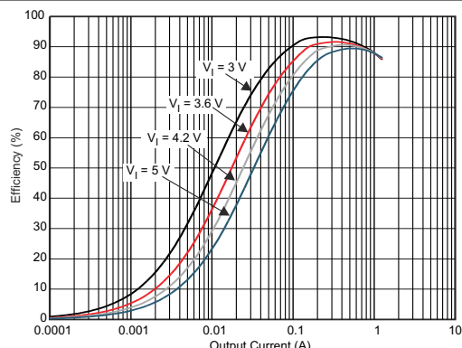
FIG 6-8. DCDC2 Efficiency vs Output Current
