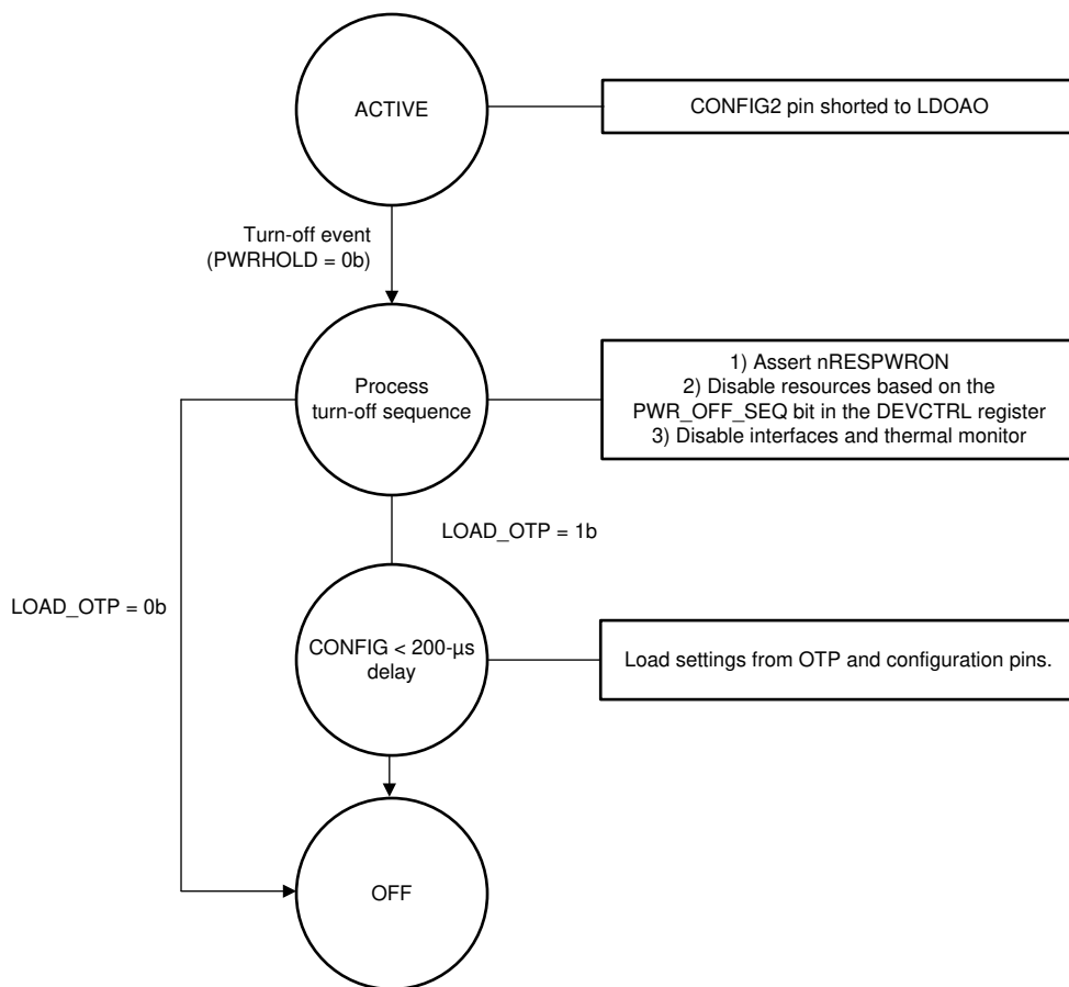
8-7. SHUTDOWN Flow for CONFIG2 Pin Shorted to LDOAO
