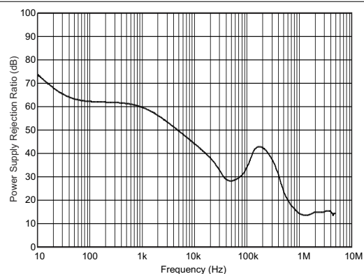
Figure 6-24. LDO4 and LDO5 PSRR vs Frequency
