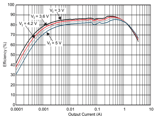
Figure 6-19. DCDC4 Efficiency vs Output Current
