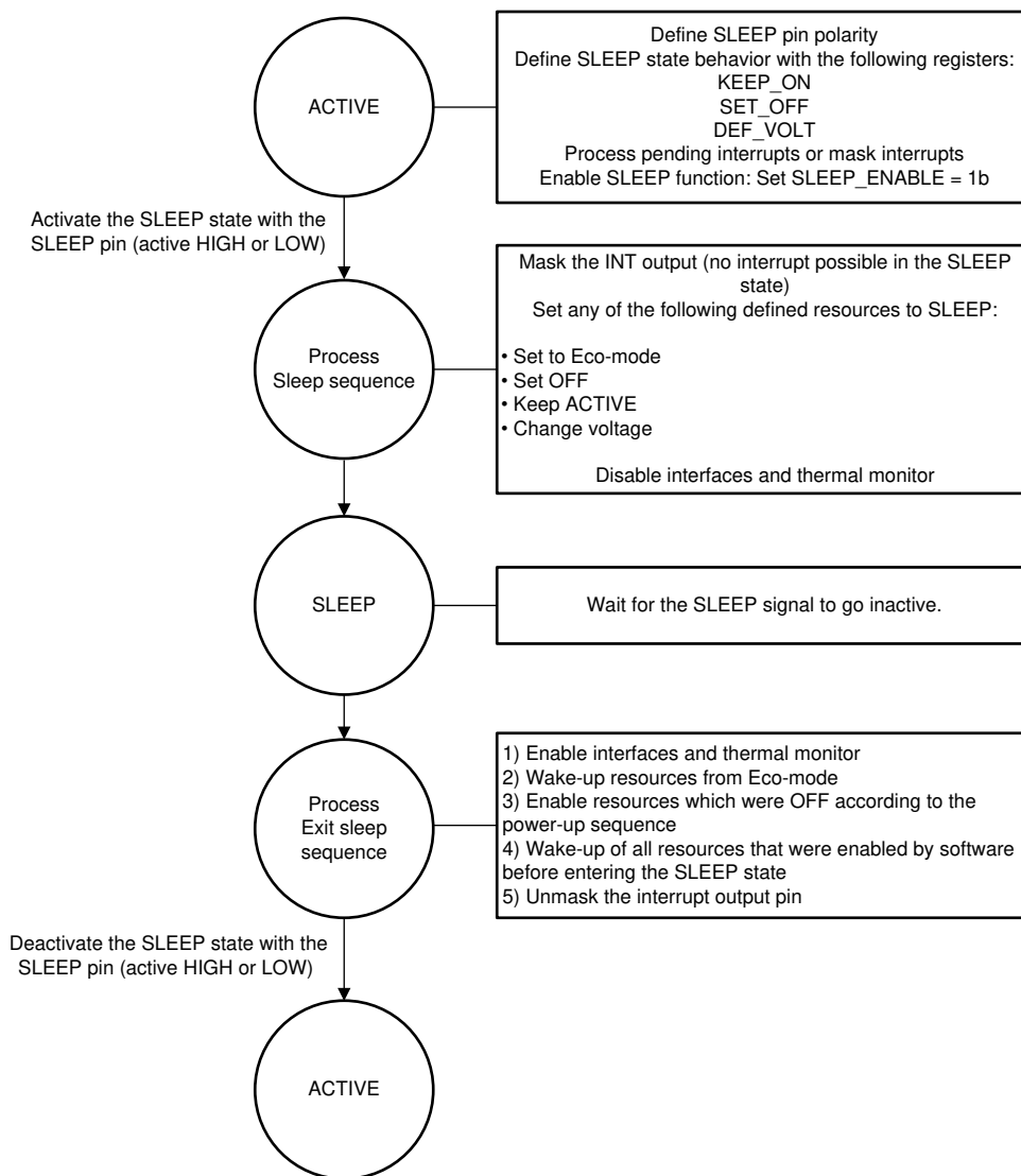
8-6. SLEEP Flow for CONFIG2 Pin Shorted LDOAO
