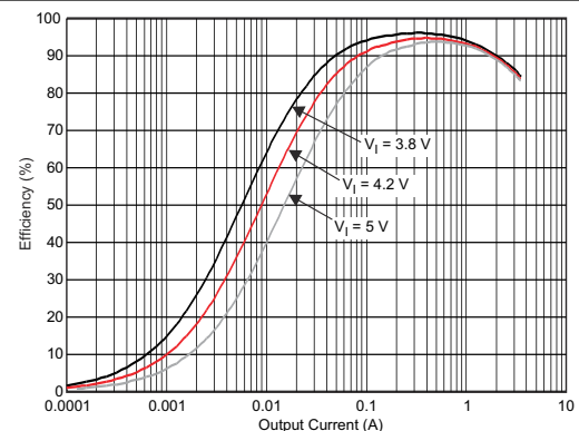
Figure 6-20. DCDC4 Efficiency vs Output Current
