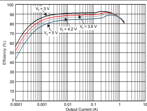
V_{OUT} = 2.1\text{ V} LQM2MPN-1R0 PFM Mode T_A = 25^\circ\text{C}
