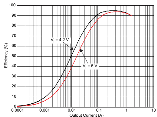
V_{OUT} = 3.2\text{ V} DEF25012-1R0 PWM Mode T_A = 25^\circ\text{C}
