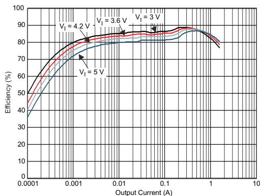
V_{OUT} = 1.1375\text{ V} DFE252012-1R0 PFM Mode T_A = 25^\circ\text{C}
