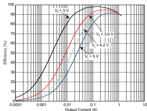
FIG 6-10. DCDC2 Efficiency vs Output Current
