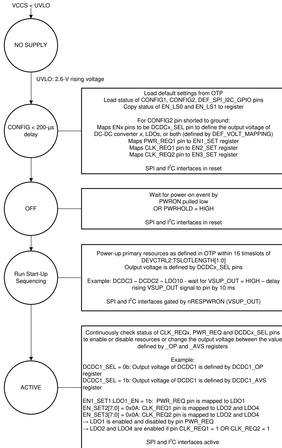
FIG 8-5. STARTUP Flow for CONFIG2 Pin Shorted to GND
