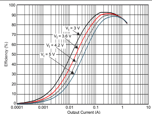
V_{OUT} = 2.1\text{ V} LQM2MPN-1R0 PWM Mode T_A = 25^\circ\text{C}
