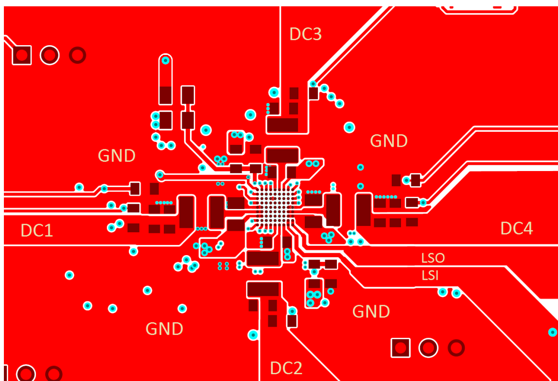
10-1. Layout Example
