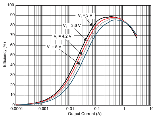
V_{OUT} = 1.1375\text{ V} PWM Mode DFE252012P-1R0 T_A = 25^\circ\text{C}
