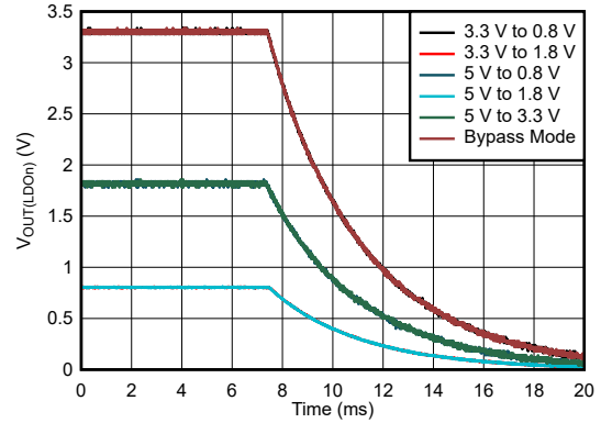
Figure 7-14. GPLDO Shutdown
