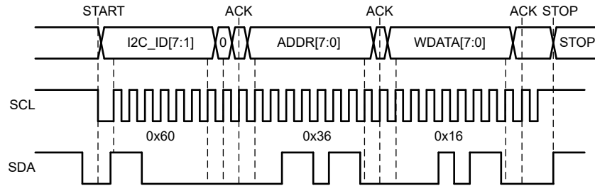
図 8-54. I 2 C Write Cycle without CRC
