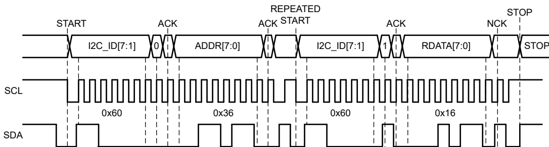
図 8-55. I 2 C Write Cycle with CRC
