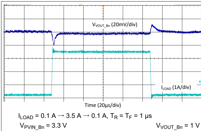
9-46. Buck Load Step Transient - 2-Phase, 2.2 MHz, Auto Mode
