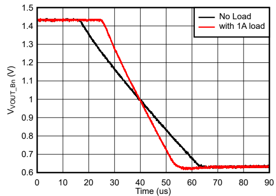
7-9. Buck Shutdown with 1A Load, Auto Mode
