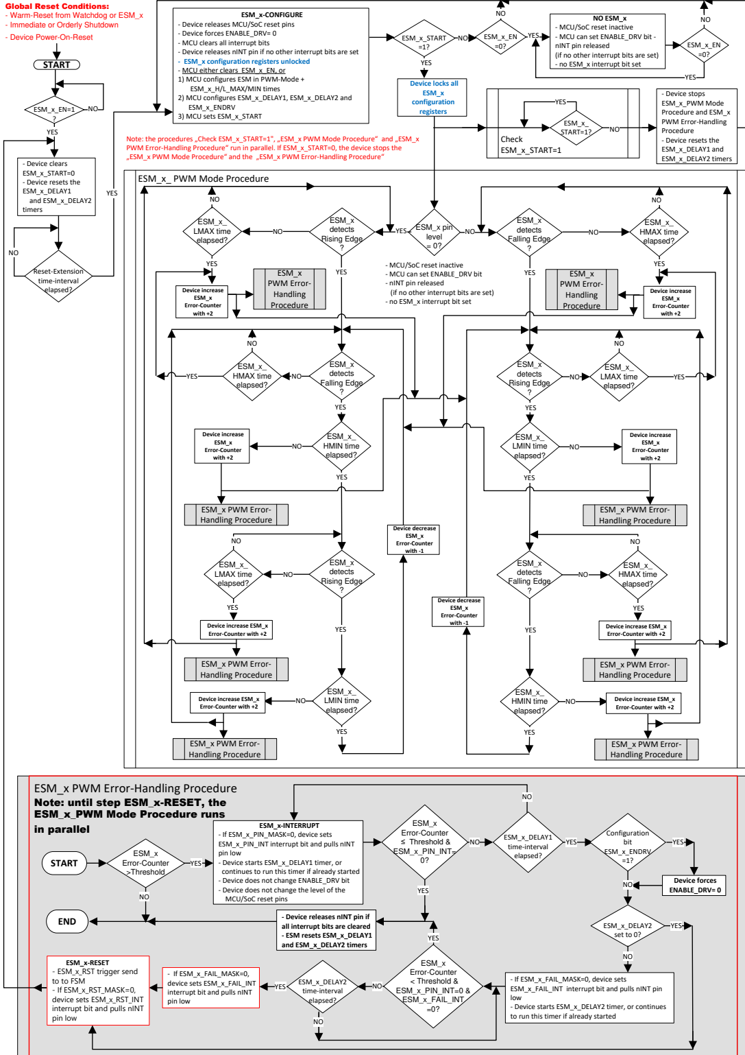
8-34. Flow-Chart for ESM_MCU and ESM_SoC in PWM Mode
