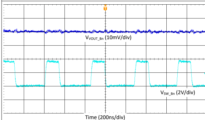
V_{PVIN\_Bn} = 3.3\text{ V} V_{VOUT\_Bn} = 1\text{ V} I_{LOAD} = 200\text{ mA} 9-26. Buck Output Ripple - 2-Phase, Fsw = 2.2 MHz, Forced-PWM Mode
