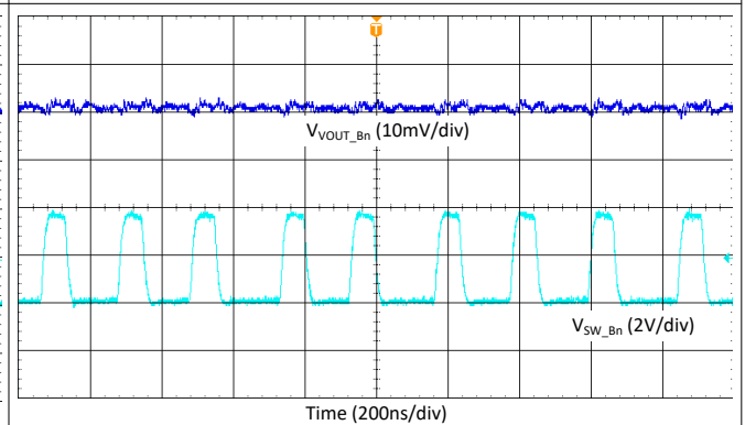
V_{PVIN\_Bn} = 3.3\text{ V} V_{VOUT\_Bn} = 1\text{ V} I_{LOAD} = 200\text{ mA} 9-27. Buck Output Ripple - 2-Phase, Fsw = 4.4 MHz, Forced-PWM Mode
