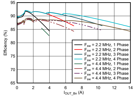
9-5. BUCK Efficiency with F_{sw} = 2.2\text{ MHz} or 4.4\text{ MHz}
