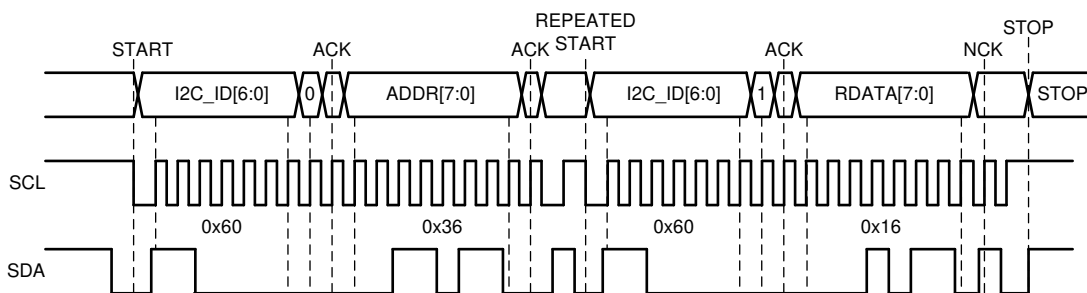
8-58. I 2 C Write Cycle with CRC
