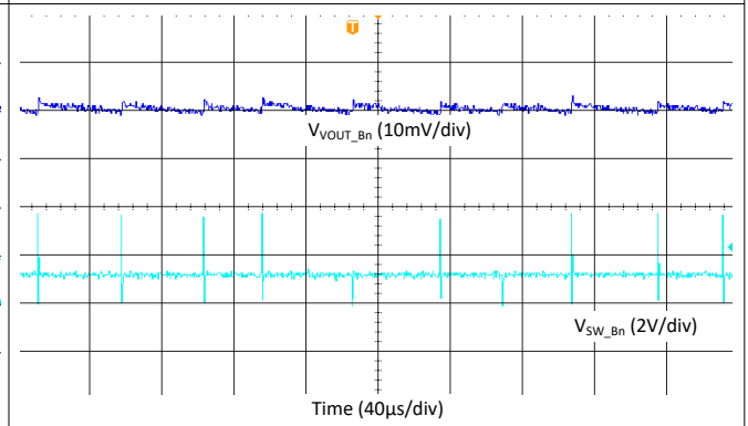
V_{PVIN\_Bn} = 3.3\text{ V} V_{VOUT\_Bn} = 1\text{ V} I_{LOAD} = 10\text{ mA} 9-25. Buck Output Ripple - 2-Phase, Auto Mode
