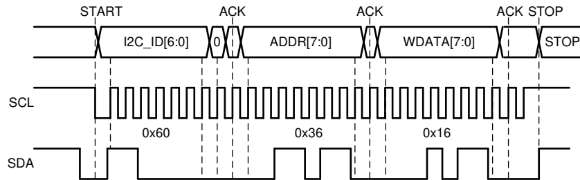
8-57. I 2 C Write Cycle without CRC
