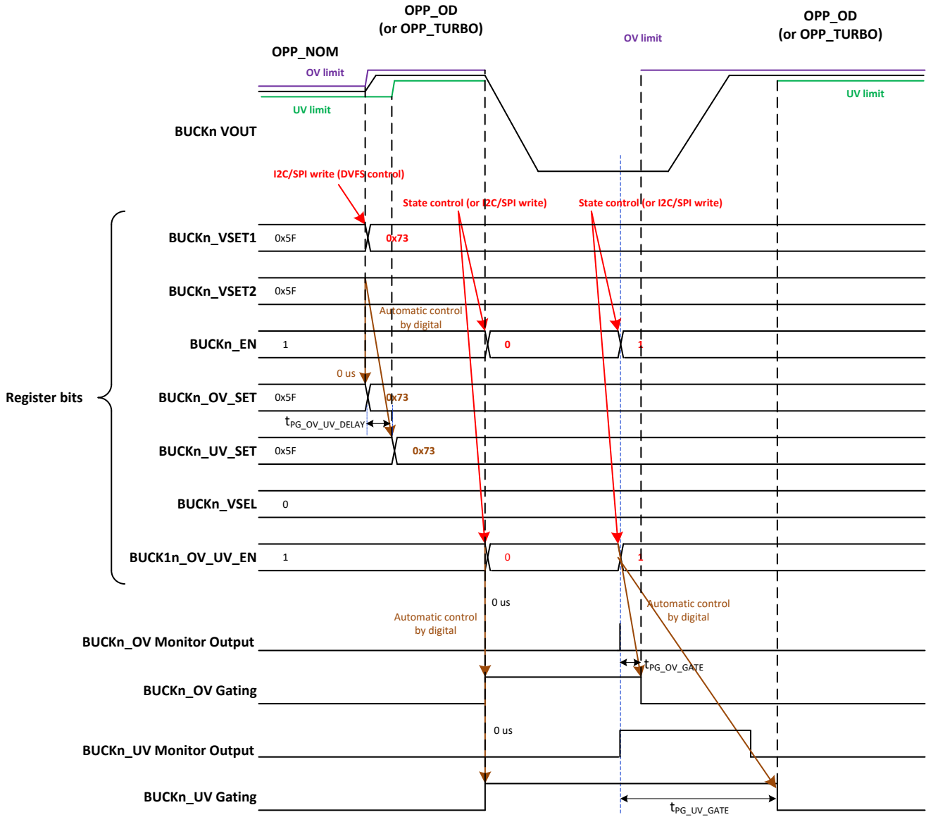
8-7. DVS Voltage and OV UV Threshold Level Change Timing Diagram
