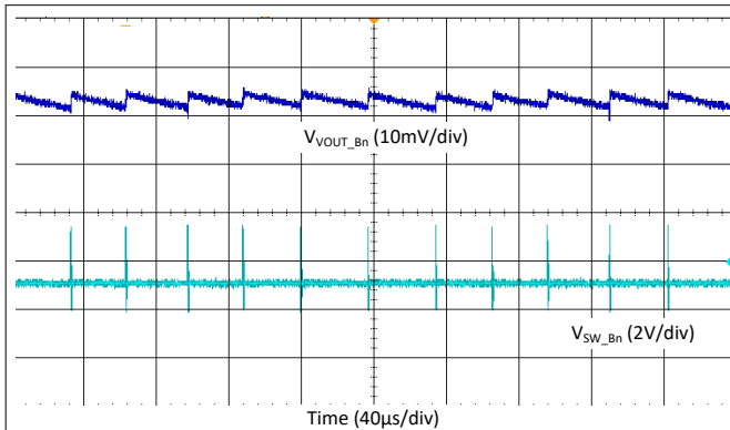
V_{PVIN\_Bn} = 3.3\text{ V} V_{VOUT\_Bn} = 1\text{ V} I_{LOAD} = 10\text{ mA} 9-22. Buck Output Ripple - Single Phase, Auto Mode
