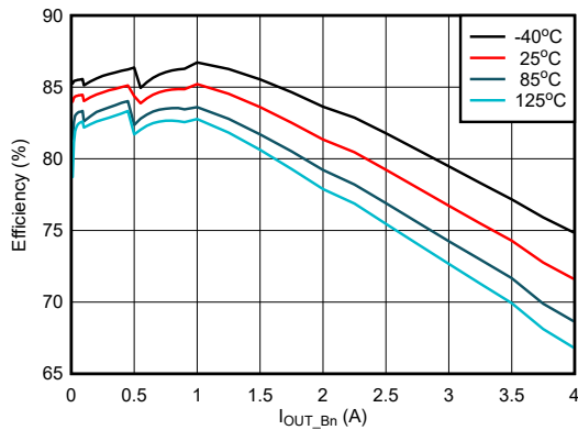
9-10. BUCK Efficiency at different T_A , Auto Mode
