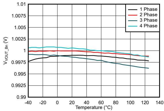
9-12. Buck Temperature Drift, Auto Mode, F_{sw} = 2.2\text{ MHz}
