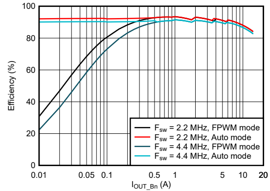
9-5. BUCK Efficiency with F_{sw} = 2.2\text{ MHz} or 4.4\text{ MHz}
