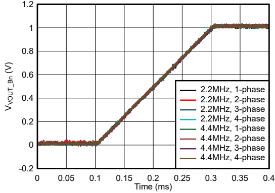
7-7. Buck Start-up with 1A Load, Auto Mode
