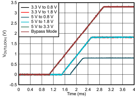
7-13. GPLDO Start-up with LDO_n_SLOW_RAMP = 1
