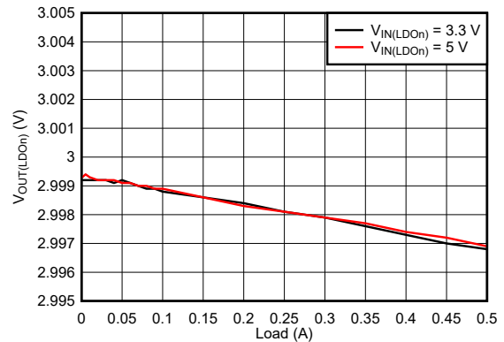
9-59. LDO1/2/3 Load Regulation, Vout = 3 V
