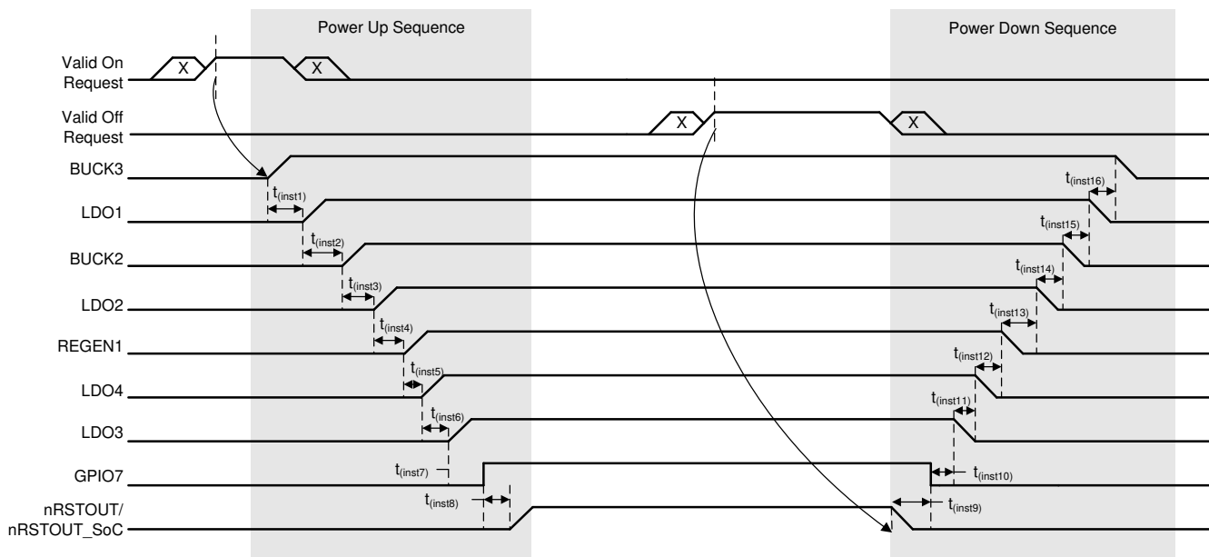
☒ 8-45. Power Sequence Example
