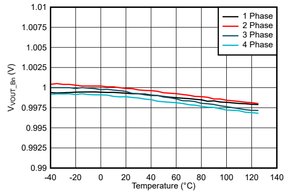
9-13. Buck Temperature Drift, Auto Mode, F_{sw} = 4.4\text{ MHz}
