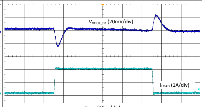
9-49. Buck Load Step Transient - 2-Phase, 4.4 MHz, Forced-PWM Mode
