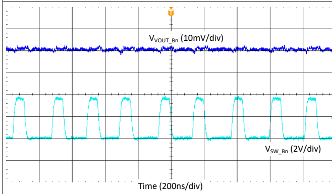
V_{PVIN\_Bn} = 3.3\text{ V} V_{VOUT\_Bn} = 1\text{ V} I_{LOAD} = 200\text{ mA} 9-24. Buck Output Ripple - Single Phase, Fsw = 4.4 MHz, Forced-PWM Mode
