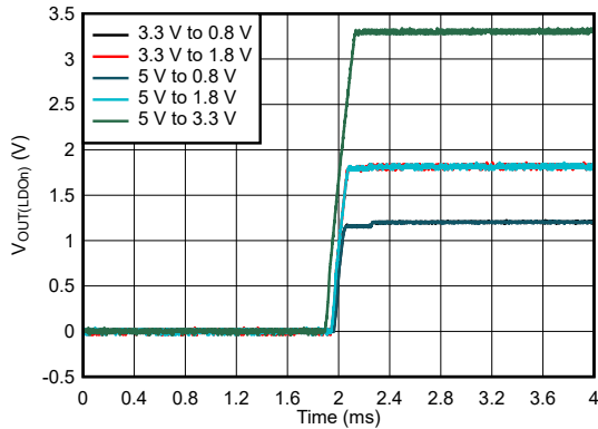
7-15. LNLDO Start-up with LDO_n_SLOW_RAMP = 0
