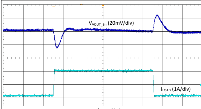
9-48. Buck Load Step Transient - 2-Phase, 2.2 MHz, Forced-PWM Mode
