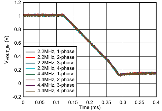
7-8. Buck Shutdown with no Load, Auto Mode
