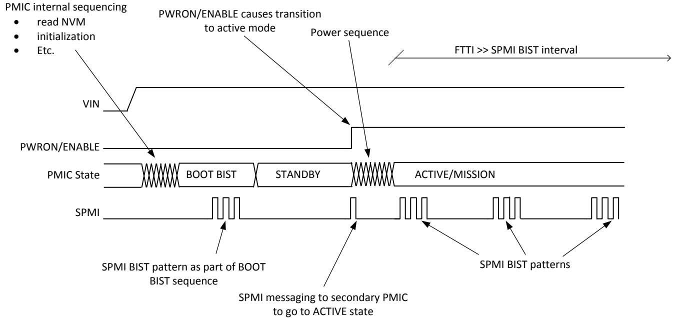
8-50. SPMI-BIST Operation
