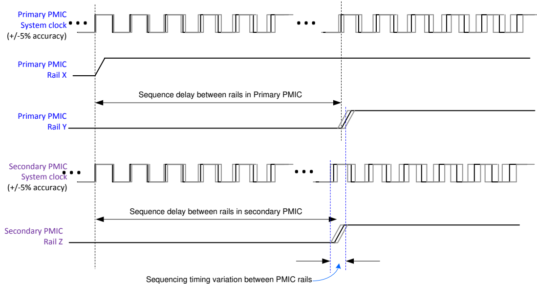
✎ 8-48. Multi-PMIC Rail Sequencing Timing Variation
