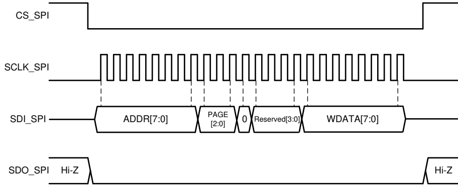
✎ 8-61. SPI Write Cycle
