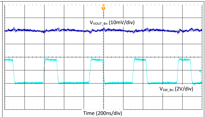
V_{PVIN\_Bn} = 3.3\text{ V} V_{VOUT\_Bn} = 1\text{ V} I_{LOAD} = 200\text{ mA} 9-23. Buck Output Ripple - Single Phase, Fsw = 2.2 MHz, Forced-PWM Mode
