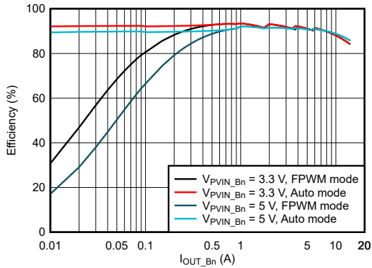
9-4. BUCK Efficiency at 3.3 V or 5 V Input Voltage
