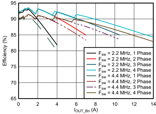
9-4. BUCK Efficiency at 3.3 V or 5 V Input Voltage
