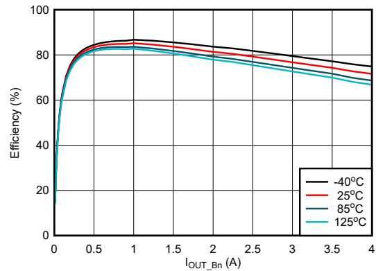
9-11. BUCK Efficiency at different T_A , Forced-PWM Mode
