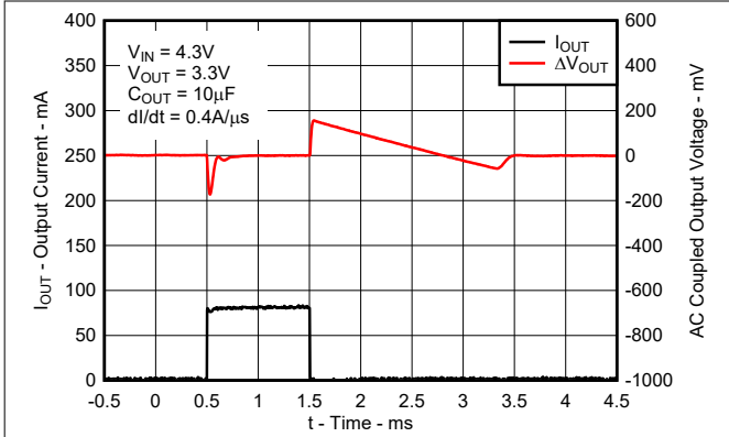
5-31. Load Transient Response (New Chip)
