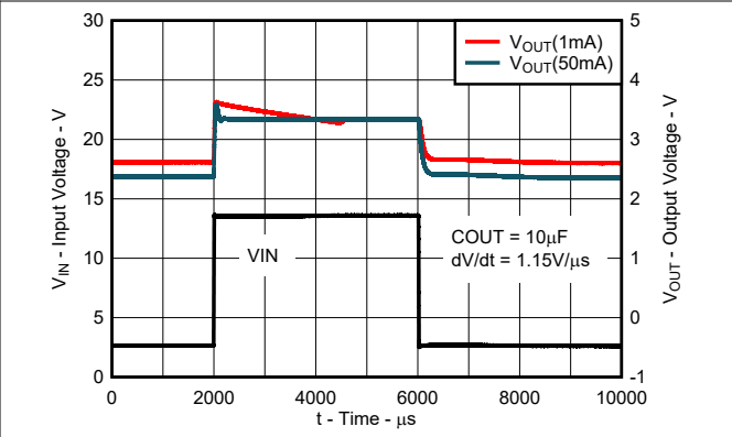
5-32. Line Transient Response (New Chip)
