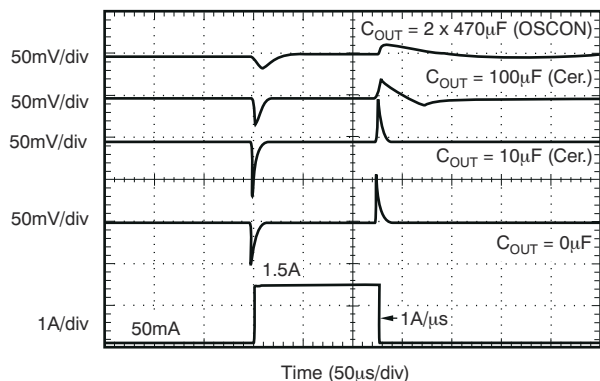
图 5-33. Output Load Transient Response (legacy chip)
