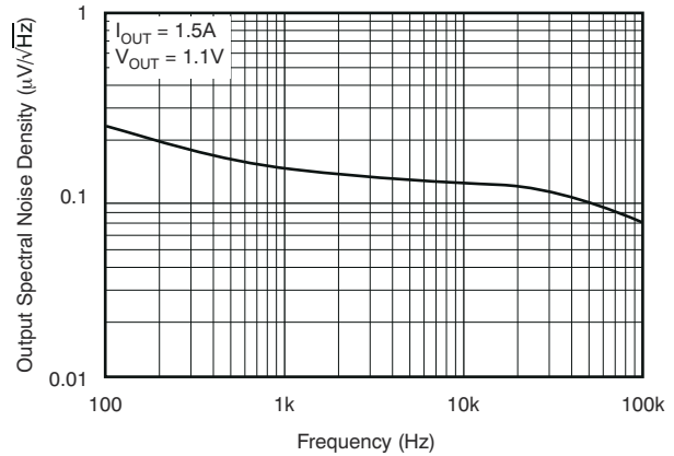
图 5-20. Noise Spectral Density (legacy chip)
