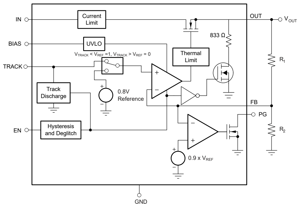
図 6-2. New chip Functional Block Diagram
