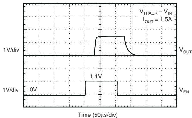
図 5-38. Turn-On Response (legacy chip)
