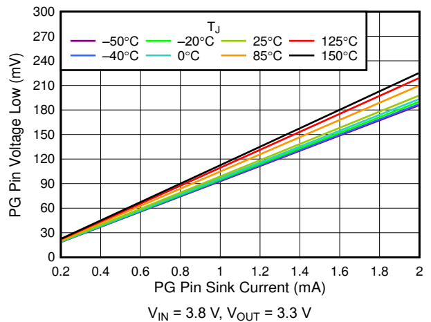
6-22. V_{OL(PG)} vs PG Pin Sink Current
