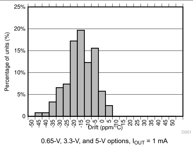
6-4. Temperature Drift Histogram ( -40^\circ\text{C} to +25^\circ\text{C} )
