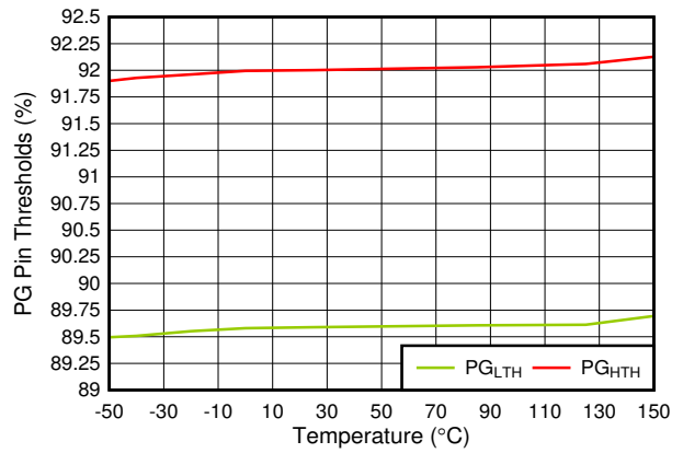
6-20. P_{GLTH} and P_{GHHTH} vs Temperature
