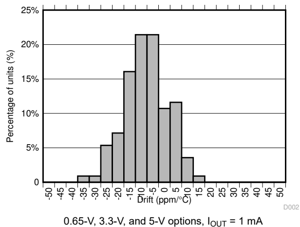
6-5. Temperature Drift Histogram ( 25^\circ\text{C} to 150^\circ\text{C} )
