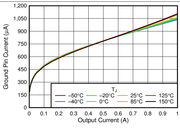
Figure 8. I_{GND} vs I_{OUT}
