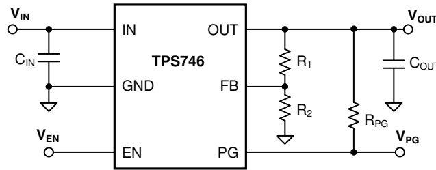
Figure 50. TPS746 Typical Application
