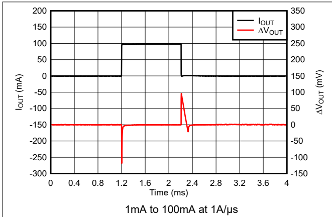
图 5-43. TPS76933 Load Transient Response (New Chip)
