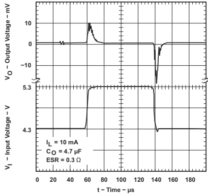
7-10. TPS76933-Q1 Line Transient Response (Legacy Chip)
