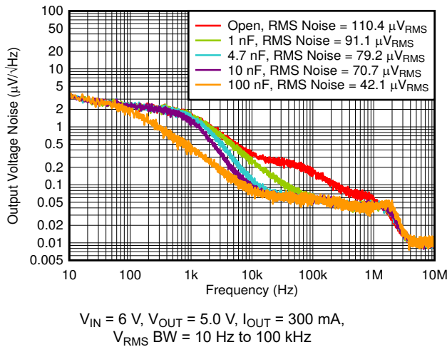
6-31. Output Noise vs Frequency and C_{FF}
