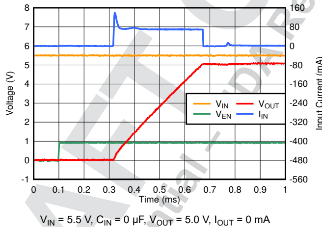
6-33. Startup Inrush Current With C_{OUT} = 4.7\text{ }\mu\text{F}
