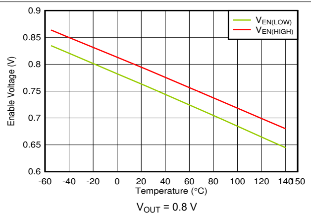
6-38. EN High and Low Threshold vs Temperature
