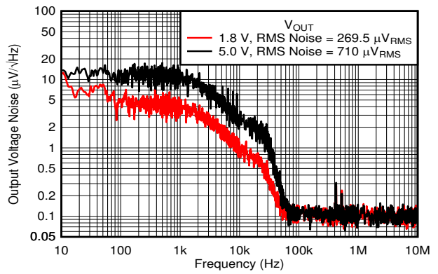
V_{IN} = V_{OUT} + 1.0\text{ V} , I_{OUT} = 1\text{ mA} , C_{OUT} = 1\text{ }\mu\text{F} 6-48. Output Noise vs Frequency and V_{OUT}
