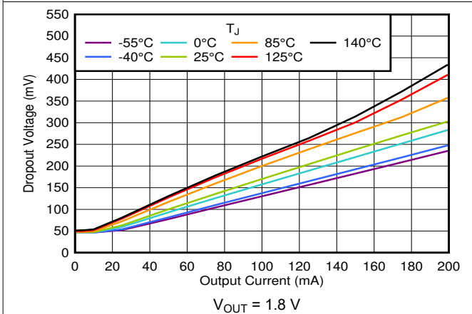
6-33. Dropout vs I_{OUT} and Temperature
