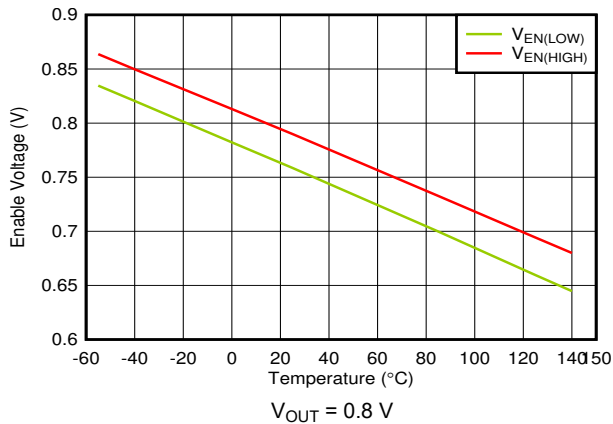
6-39. EN High and Low Threshold vs Temperature
