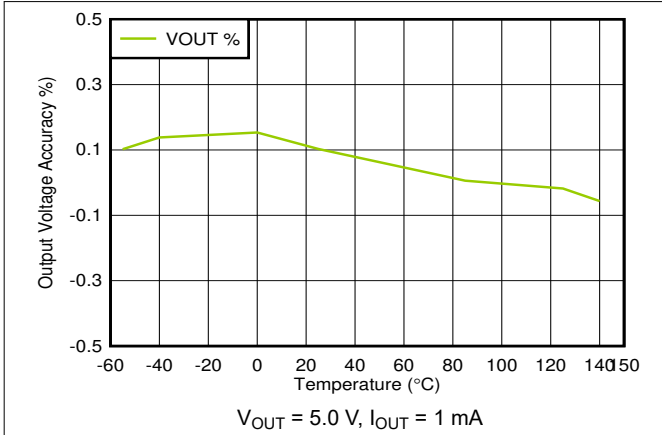
6-31. Output Accuracy vs Temperature
