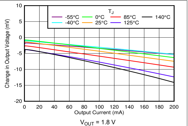
6-32. Load Regulation vs V_{IN} and Temperature
