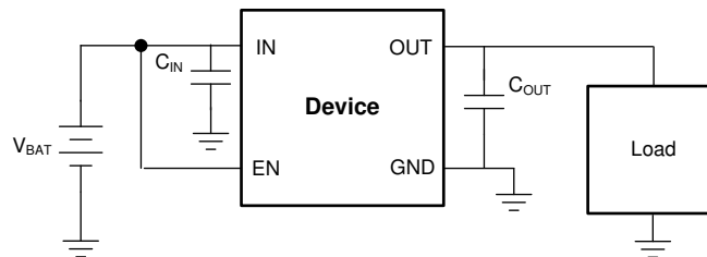
☒ 8-4. Operation From a Battery Input Supply
