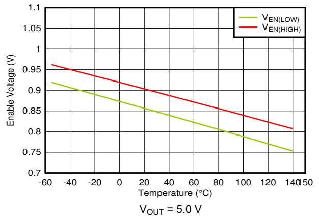
6-40. EN High and Low Threshold vs Temperature
