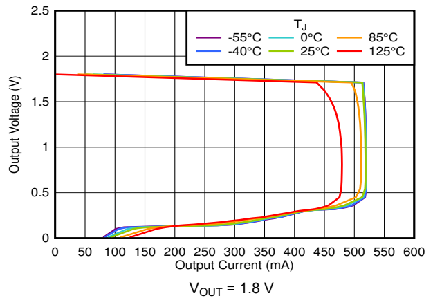
6-38. Foldback Current Limit vs I_{OUT} and Temperature
