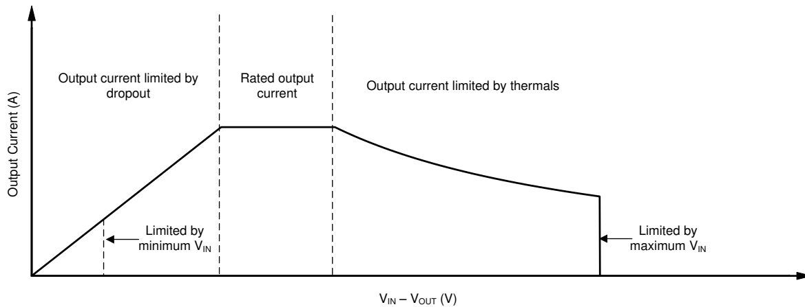
☒ 8-3. Region Description of Continuous Operation Regime
