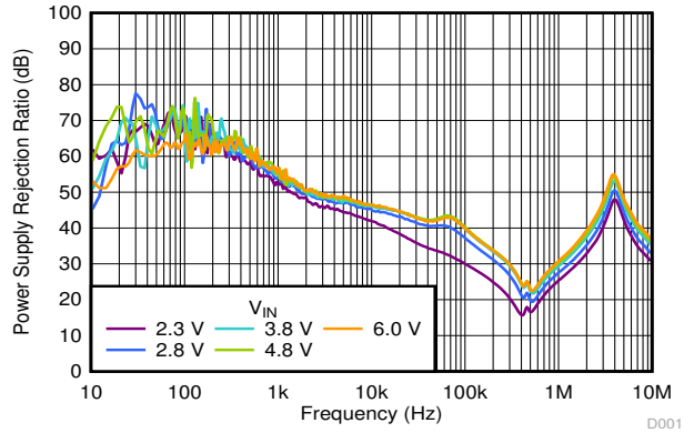
V_{OUT} = 1.8\text{ V} , I_{OUT} = 100\text{ mA} , C_{OUT} = 1\text{ }\mu\text{F} 6-46. PSRR vs Frequency and V_{IN}
