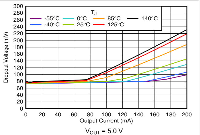
6-34. Dropout vs I_{OUT} and Temperature
