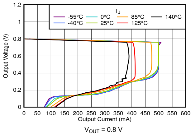
6-37. Foldback Current Limit vs I_{OUT} and Temperature
