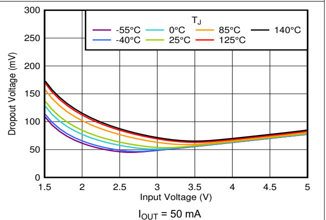
6-36. Dropout vs V_{IN} and Temperature
