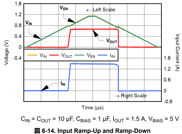
FIG 6-14. Input Ramp-Up and Ramp-Down
