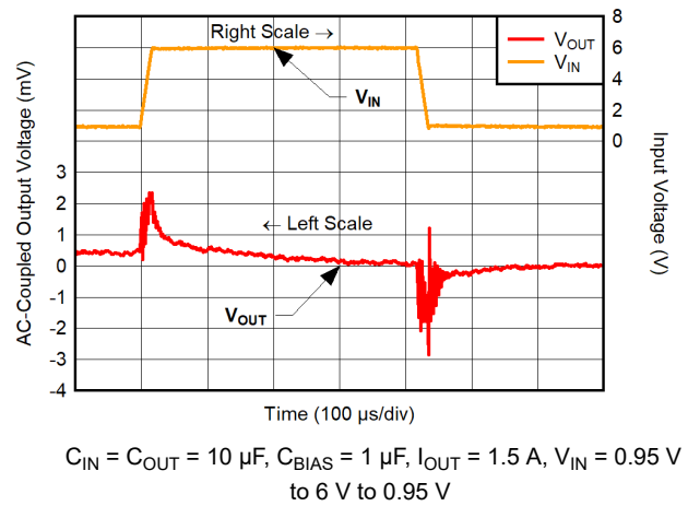
FIG 6-12. Line Transient for V_{OUT} = 0.65\text{ V}
