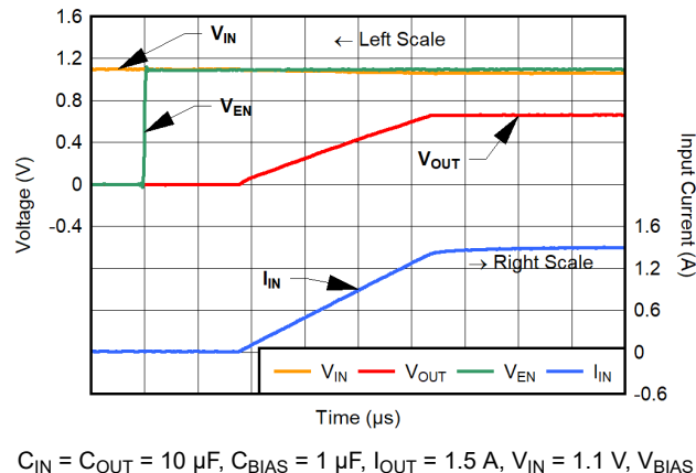
FIG 6-15. Input Ramp With Fast Soft-Start
