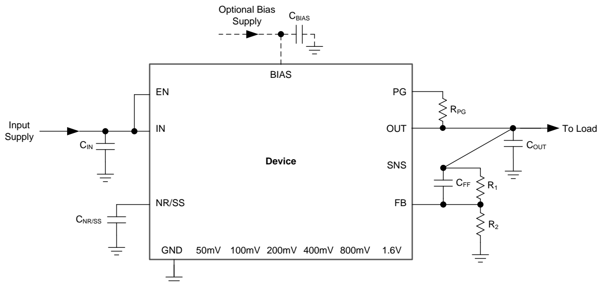
Figure 68. Typical Application
