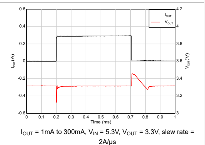
Figure 5-36. Load Transient
