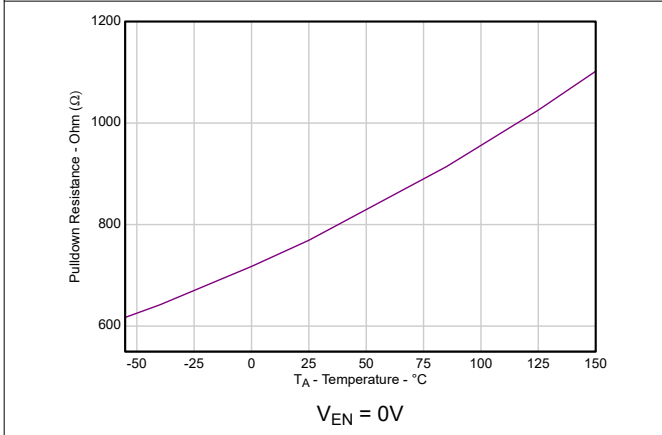
Figure 5-27. Output Discharge Resistance vs Temperature
