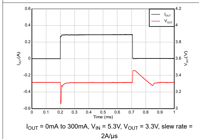
Figure 5-35. Load Transient
