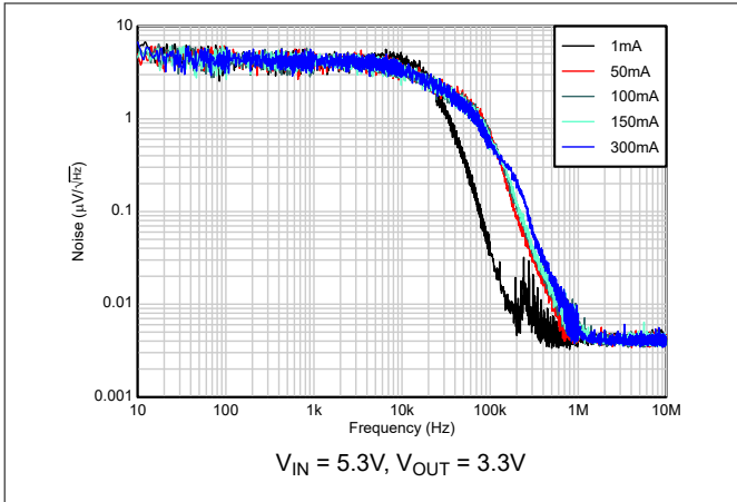
Figure 5-25. Output Noise vs Frequency, Output Current
