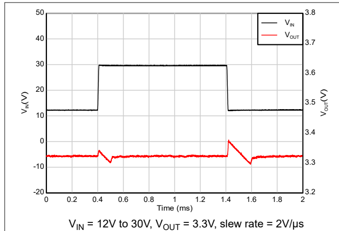
Figure 5-31. Line Transient
