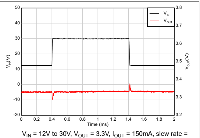
Figure 5-32. Line Transient
