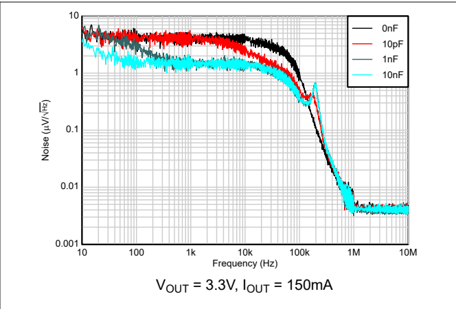
Figure 5-26. Output Noise vs Frequency, C_{FF}
