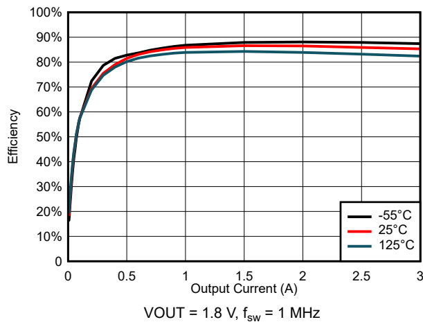
图 6-55. Efficiency for V_{\text{IN}} = 5.5\ \text{V}
