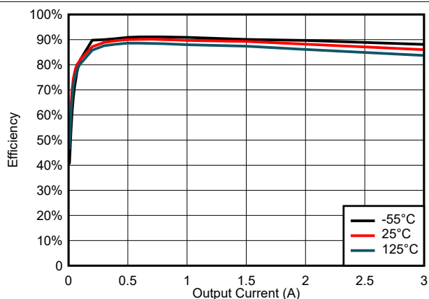
Figure 6-24. Efficiency for V_{\text{IN}} = 3\ \text{V}
