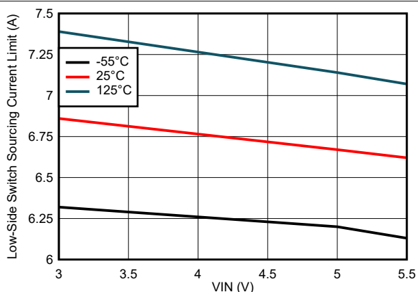
6-12. Low-Side Switch Sourcing Current Limit Variation
