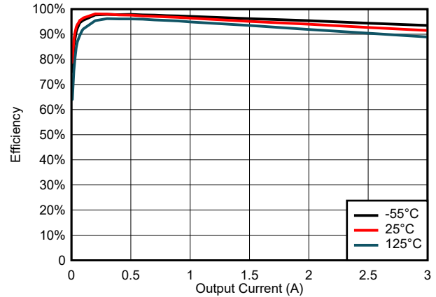
FIG 6-18. Efficiency for V_{\text{IN}} = 3\ \text{V}
