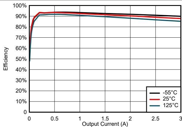
FIG 6-19. Efficiency for V_{\text{IN}} = 3\ \text{V}
