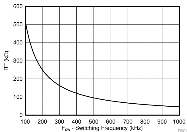
図 7-4. RT vs Switching Frequency
