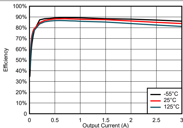
Figure 6-23. Efficiency for V_{\text{IN}} = 3\ \text{V}
