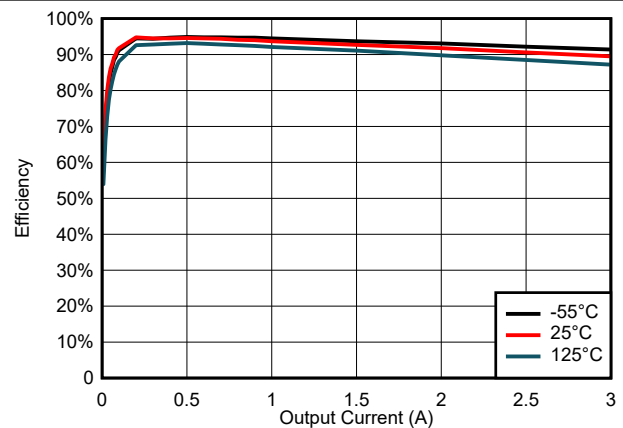
FIG 6-20. Efficiency for V_{\text{IN}} = 3\ \text{V}
