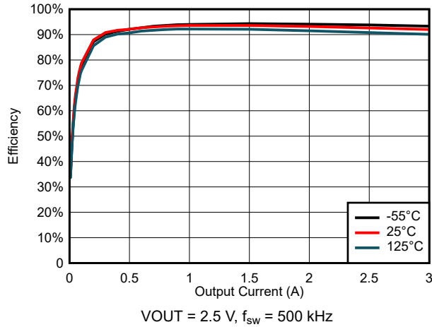
图 6-53. Efficiency for V_{\text{IN}} = 5.5\ \text{V}
