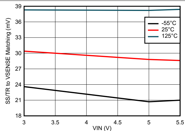
6-10. SS/TR to VSENSE Matching Variation
