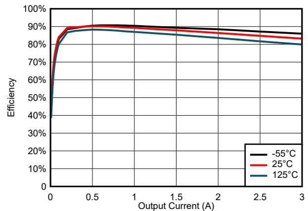
FIG 6-18. Efficiency for V_{\text{IN}} = 3\ \text{V}
