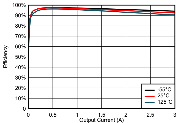
FIG 6-17. Efficiency for V_{\text{IN}} = 3\ \text{V}
