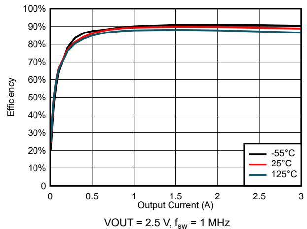
图 6-56. Efficiency for V_{\text{IN}} = 5.5\ \text{V}
