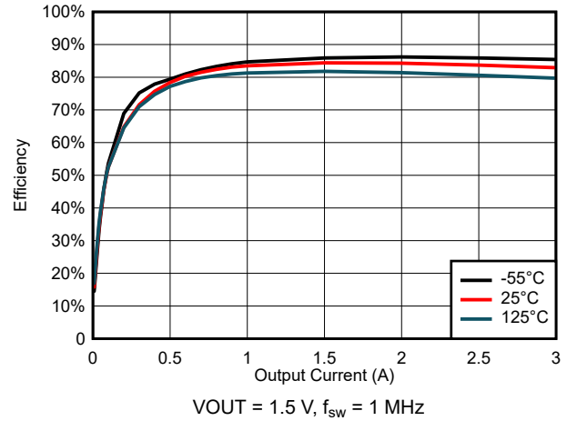
图 6-54. Efficiency for V_{\text{IN}} = 5.5\ \text{V}
