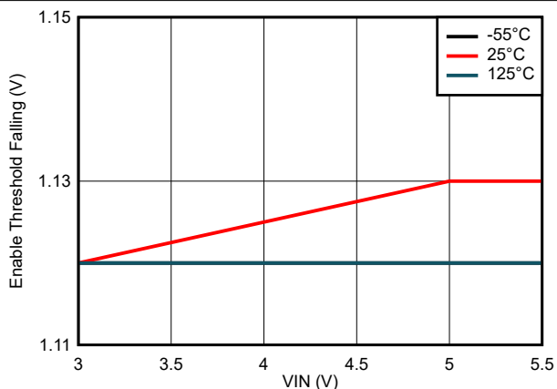
6-8. Enable Threshold Falling Variation
