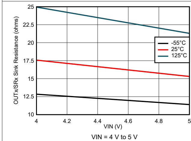
Figure 7-63. Output Sink Resistance Variation
