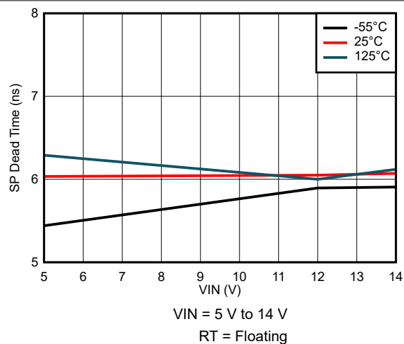
7-50. SP Dead Time Variation
