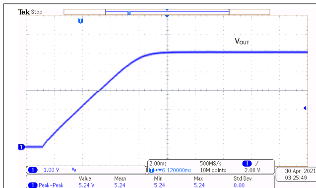
図 9-2. V_{OUT} Soft-Start of Push-Pull Converter With I_{OUT} = 10\text{ A}
