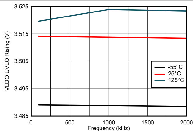
図 7-5. VLDO UVLO Rising Variation
