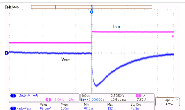
図 9-3. 5-A Load Step Response for Push Pull Converter
