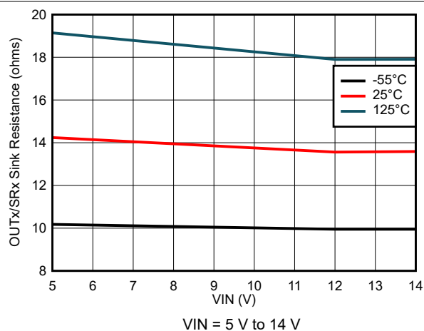
FIG 7-64. Output Sink Resistance Variation
