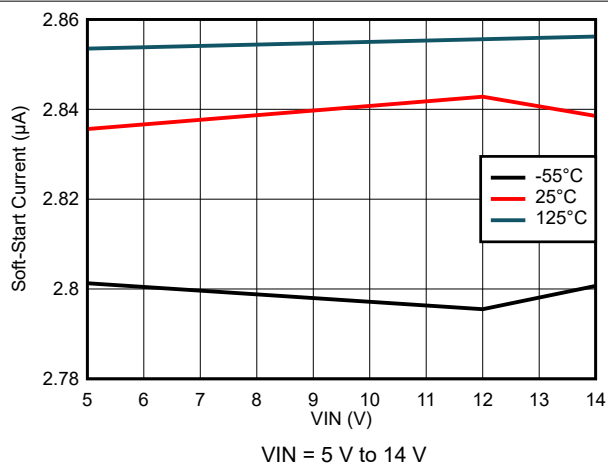
FIG 7-10. Soft-Start Current Variation
