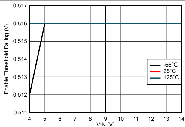
FIG 7-8. Enable Threshold Falling Variation
