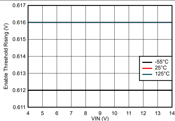
FIG 7-7. Enable Threshold Rising Variation
