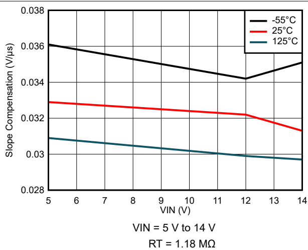
FIG 7-66. Slope Compensation Variation
