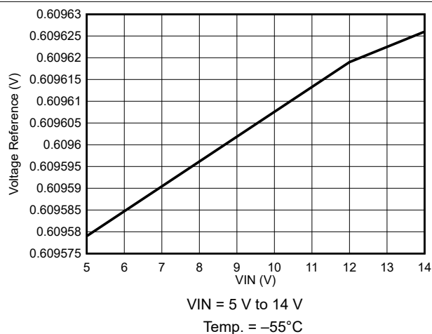
FIG 7-12. Voltage Reference Variation
