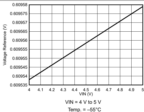
FIG 7-11. Voltage Reference Variation
