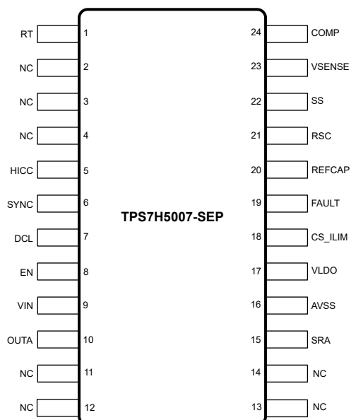
6-3. TPS7H5007-SEP PW Package 24-Pin TSSOP (Top View)
