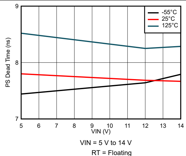
7-42. PS Dead Time Variation
