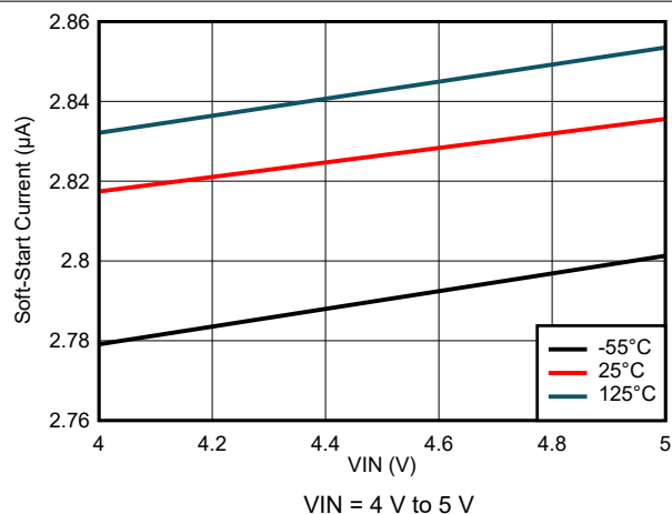
FIG 7-9. Soft-Start Current Variation
