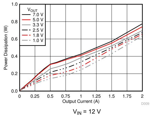
6-8. Power Dissipation versus Output Current
