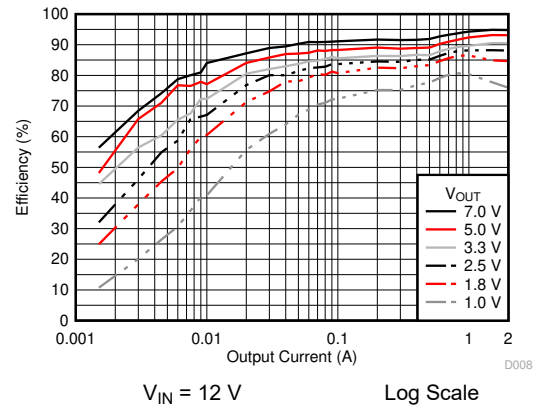
6-7. Efficiency versus Output Current
