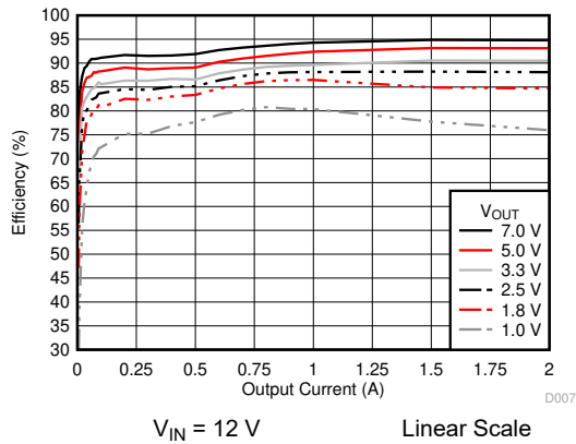
6-6. Efficiency versus Output Current
