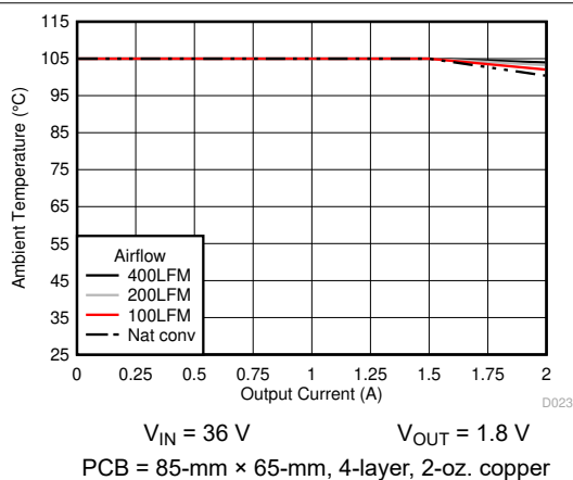
6-21. Safe Operating Area
