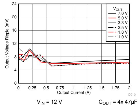
6-9. Voltage Ripple versus Output Current
