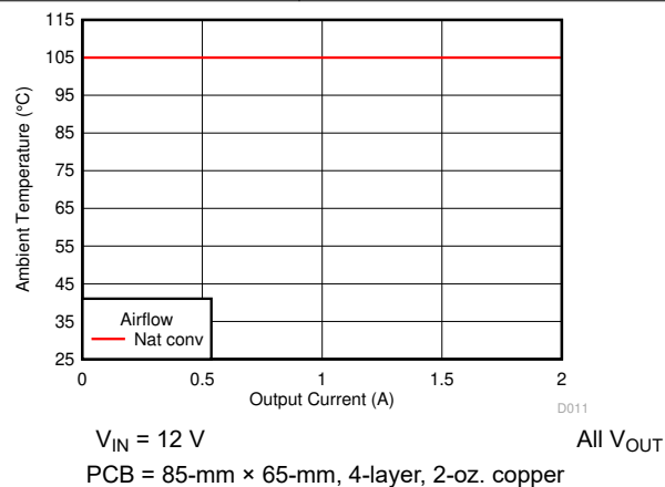
6-10. Safe Operating Area
